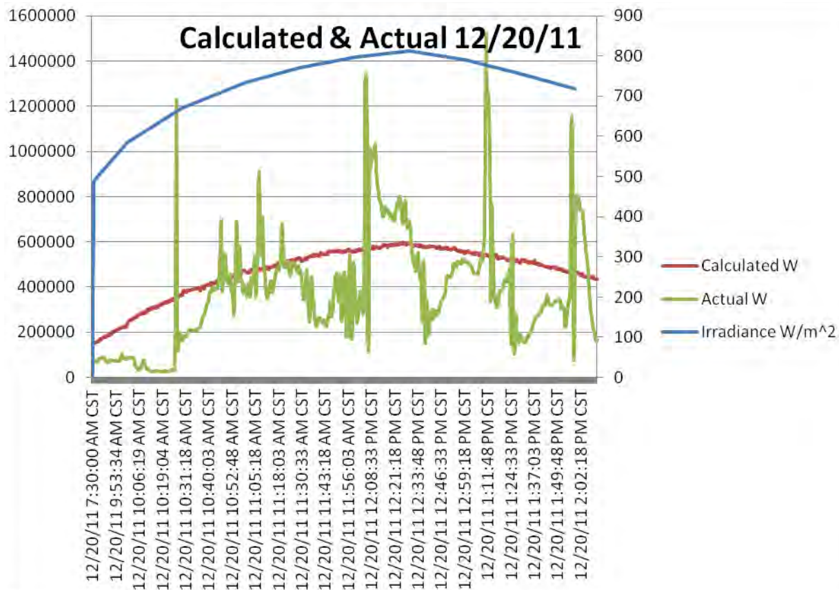
Figure A-103. Calculate and actual for 12/20/2011.
