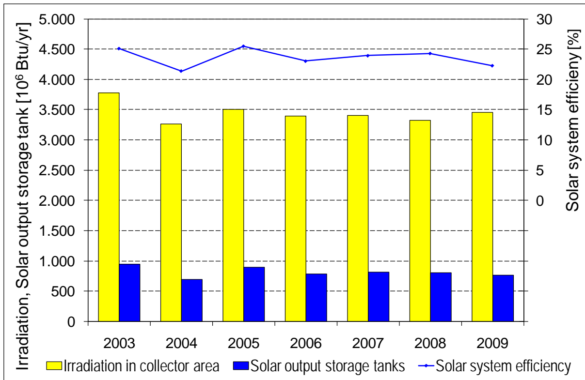
Figure A-58. Irradiation in collector area, solar energy output from the solar storage tank, and solar system efficiency.
