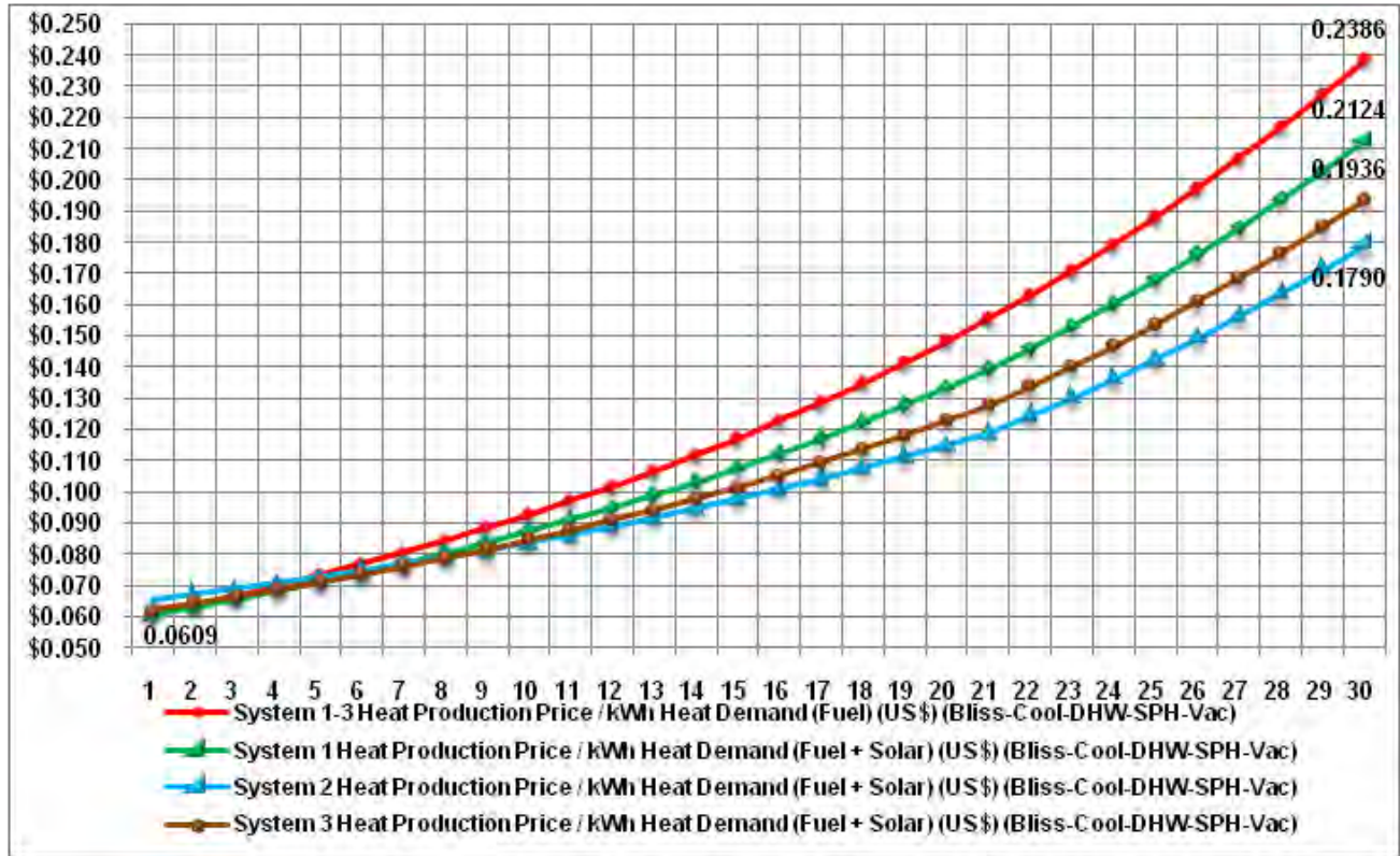
Figure B-26. Energy cost - Fort Bliss – DHW / SPH / cooling – vacuum tube collectors.
