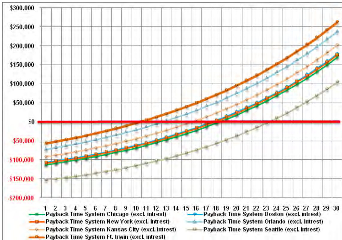
Figure C-5. Comparison of payback time scenario 2 – climate zones.
