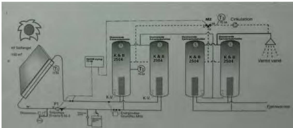
Figure A-27. Diagram of the heating system.
