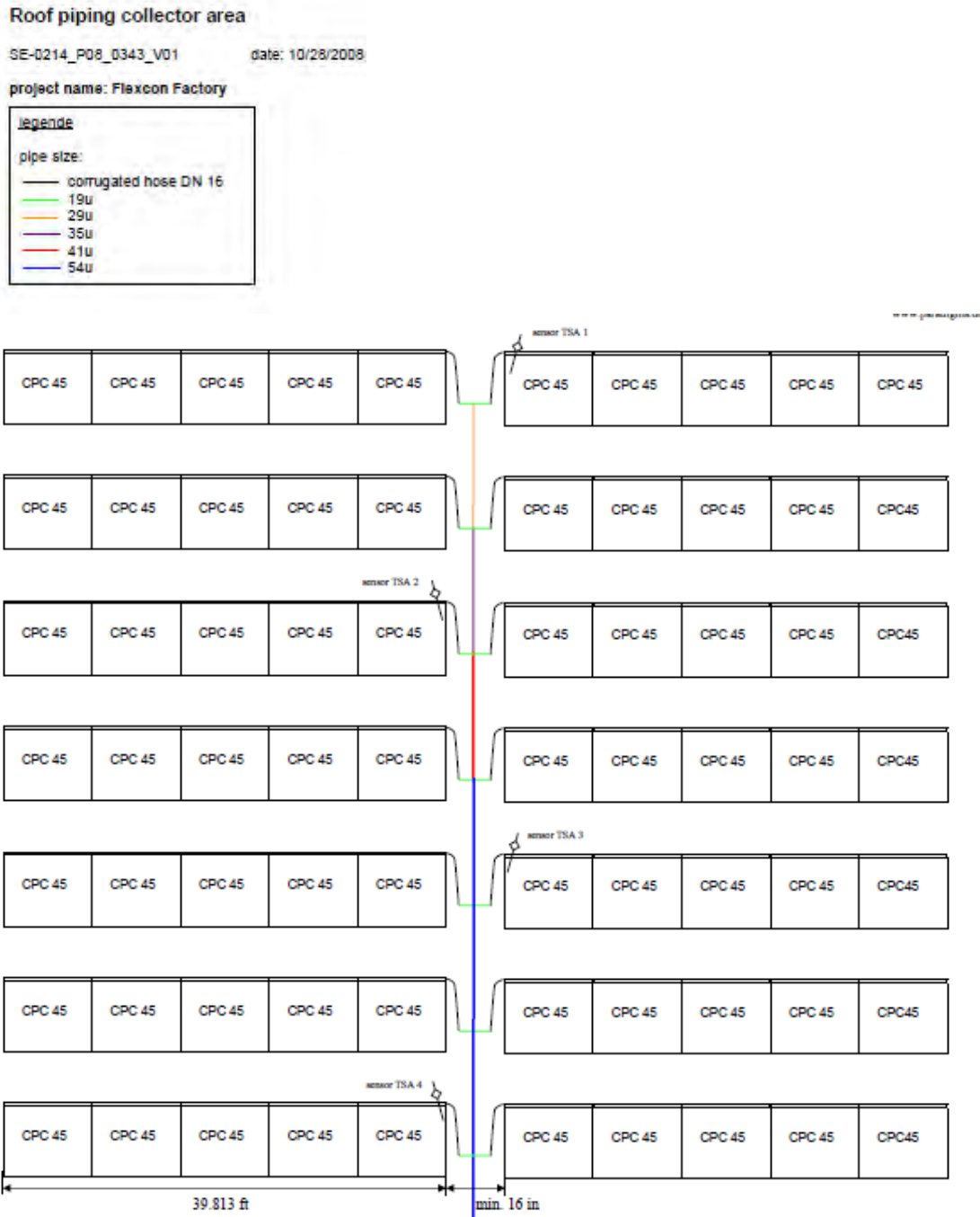
Figure 5.9. Pipe sizes used in a reversed return piping system.
