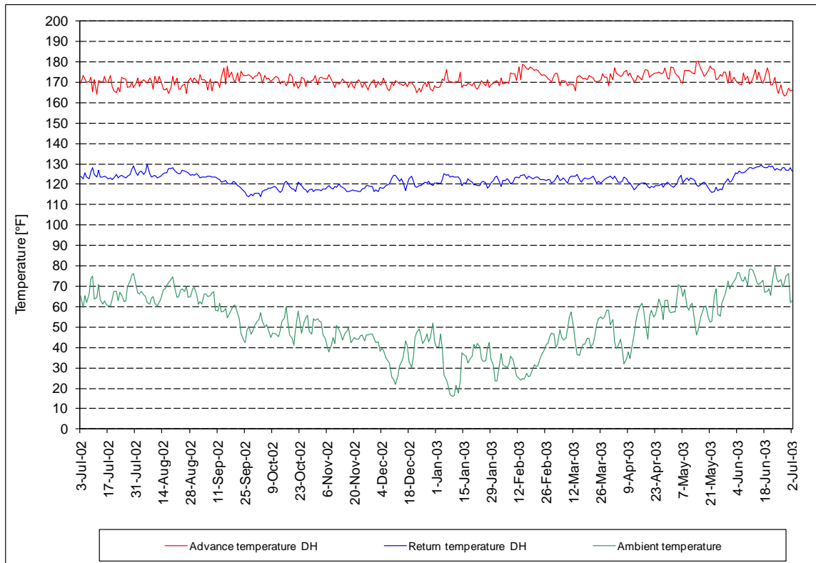
Figure A-85. Volume flow DH, volume flow through solar storage tank, and temperatures DH.
