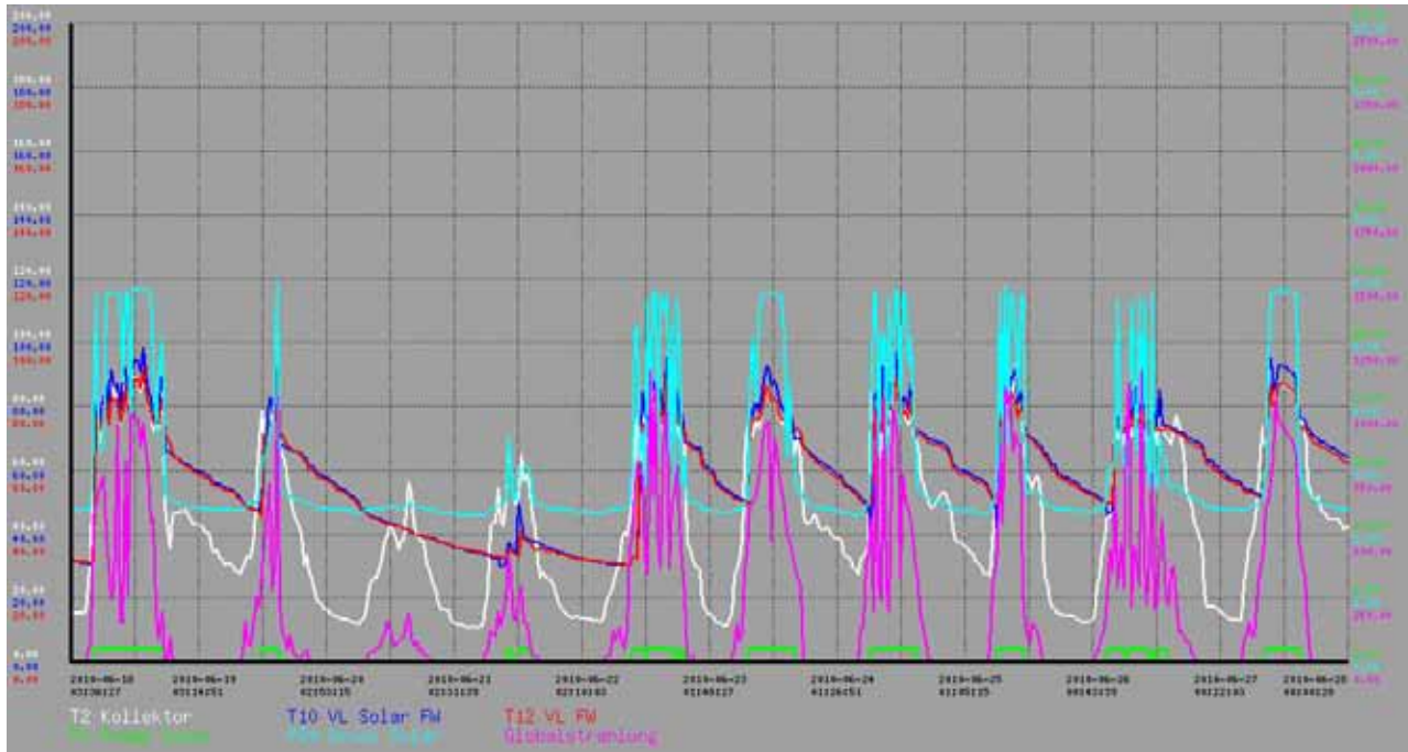
Figure A-16. Operating characteristics of the solar thermal system connected to the district heating network Water works Andritz Graz, Styria.
