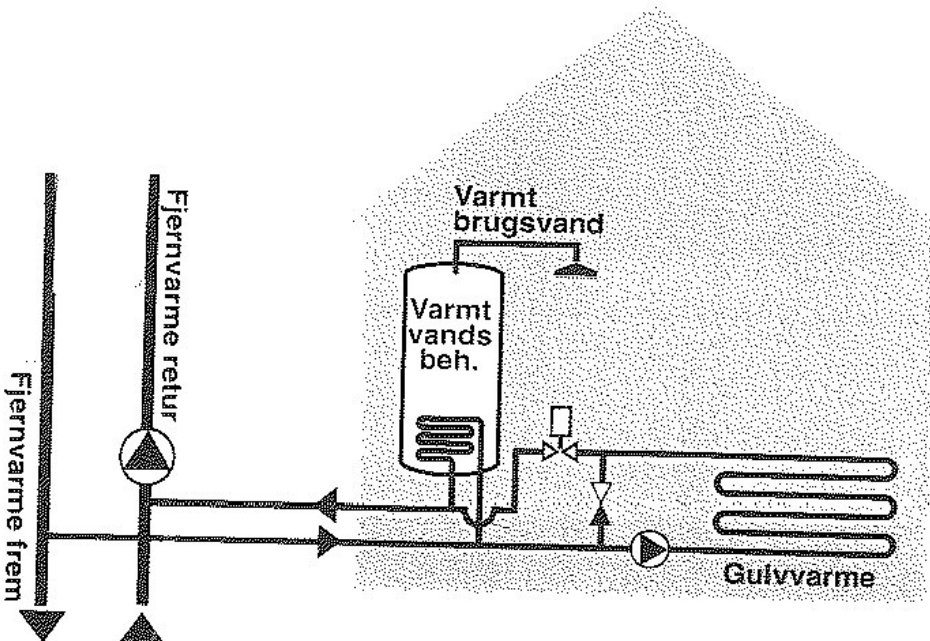
Figure A-30. Diagram of house installation.
