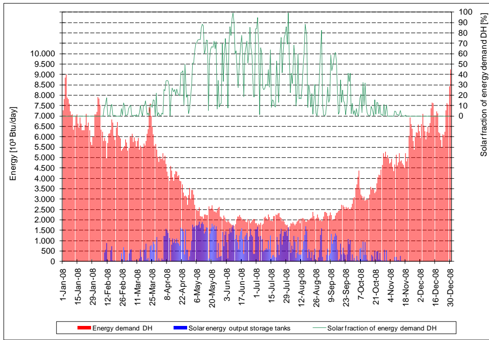
Figure A-52. Energy demand DH, energy output solar system, and solar fraction measured in 2008.
