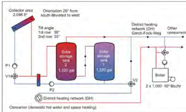
Figure A-49. Highly simplified schematics of the solar system, solar storage tanks arrangement and the integration in the district heating network (DH).
