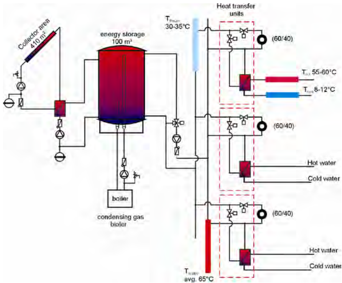
Figure A-6. Solar supported heating grid with weekly storage and two-pipe network connected to decentralized heat transfer units in Gneis-Moos, Salzburg.
