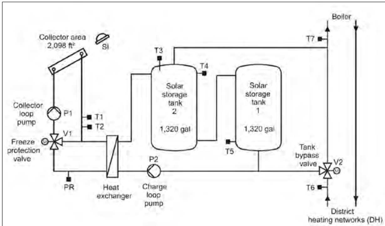
Figure A-51. Highly simplified schematics showing the positioning of the control sensors.
