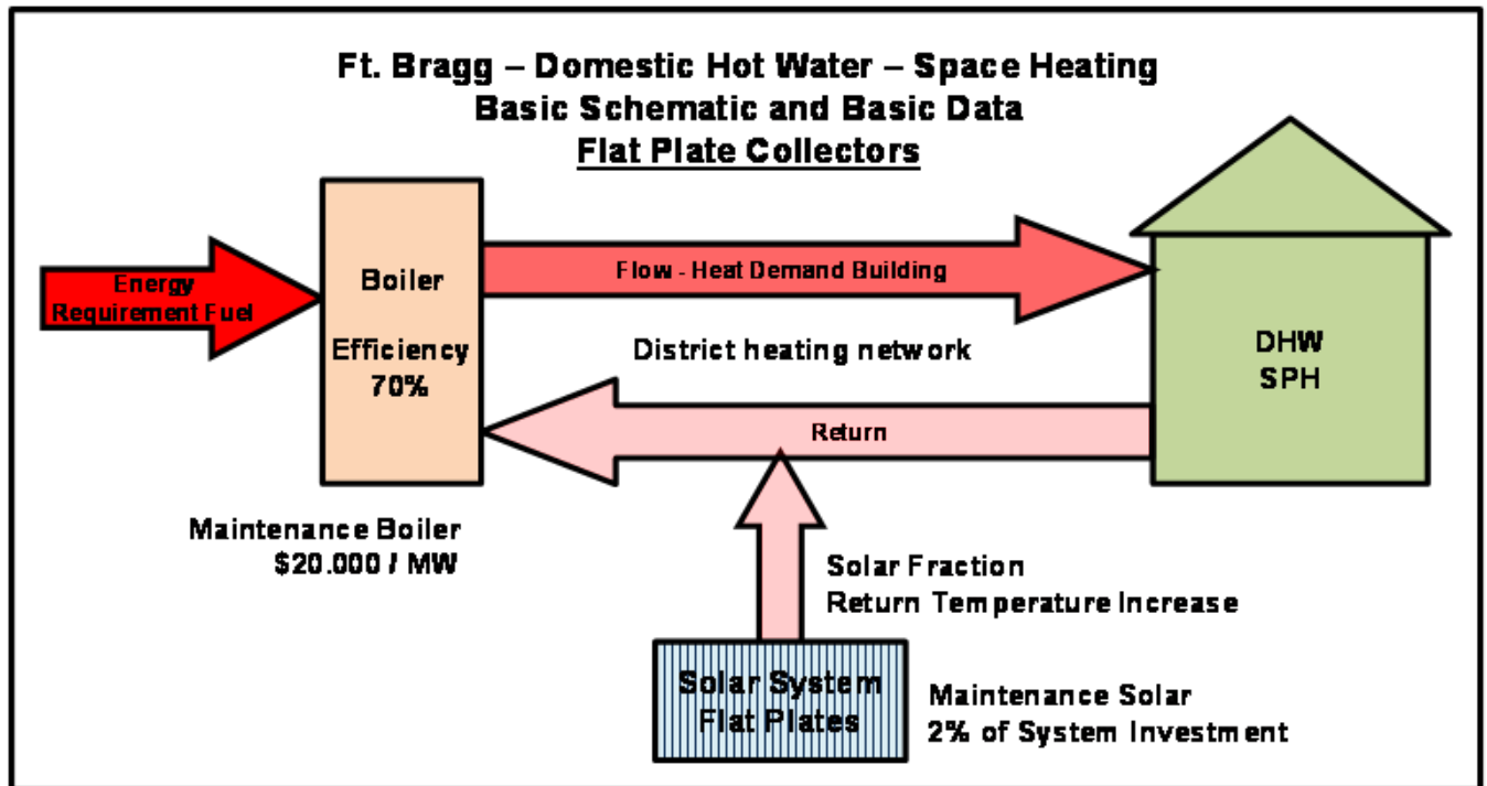
Figure B-39. Basic schematic – Fort Bragg – DHW / SPH – flat plate collectors.
