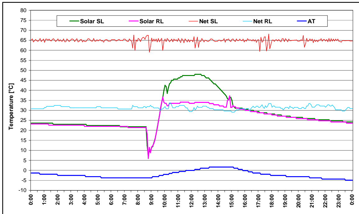
Figure A-10. Temperatures of the solar loop and the distribution grid in December 9 th 2001, Gneis-Moos.
