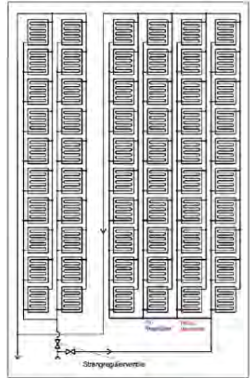
Figure A-37. Piping schematic of the facade collector field (Apartment House Frankfurt).
