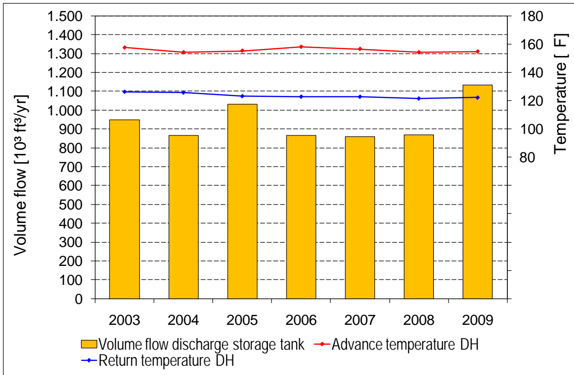
Figure A-59. Volume flow discharge solar storage tank, advance and return temperature DH.
