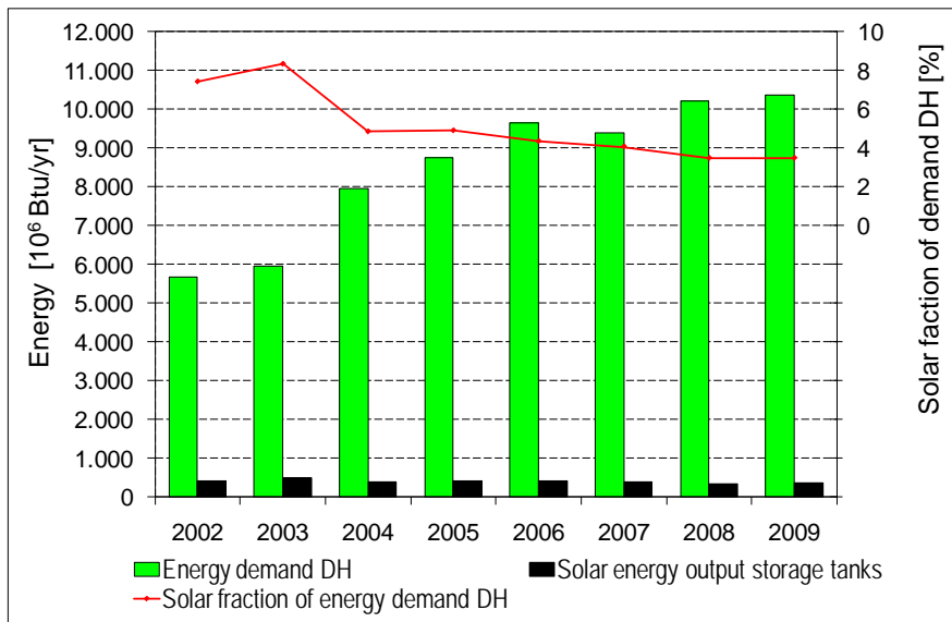
Figure A-67. Energy demand DH, solar energy output from solar storage tanks and solar fraction of total energy demand DH.
