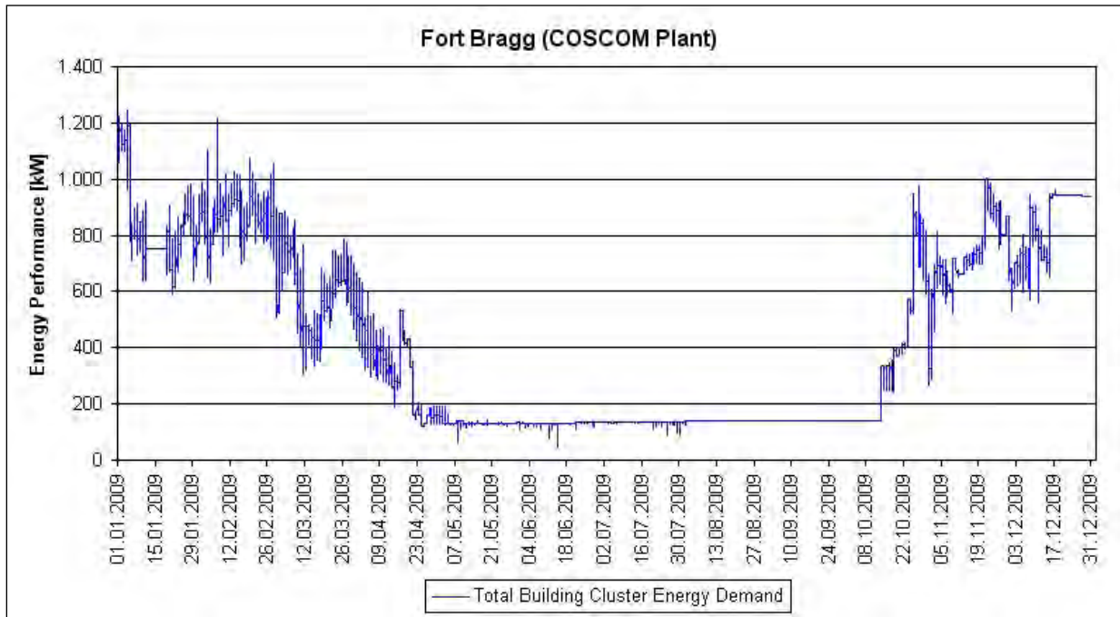
Figure B-17. Metered energy data from COSCOM Plant.
