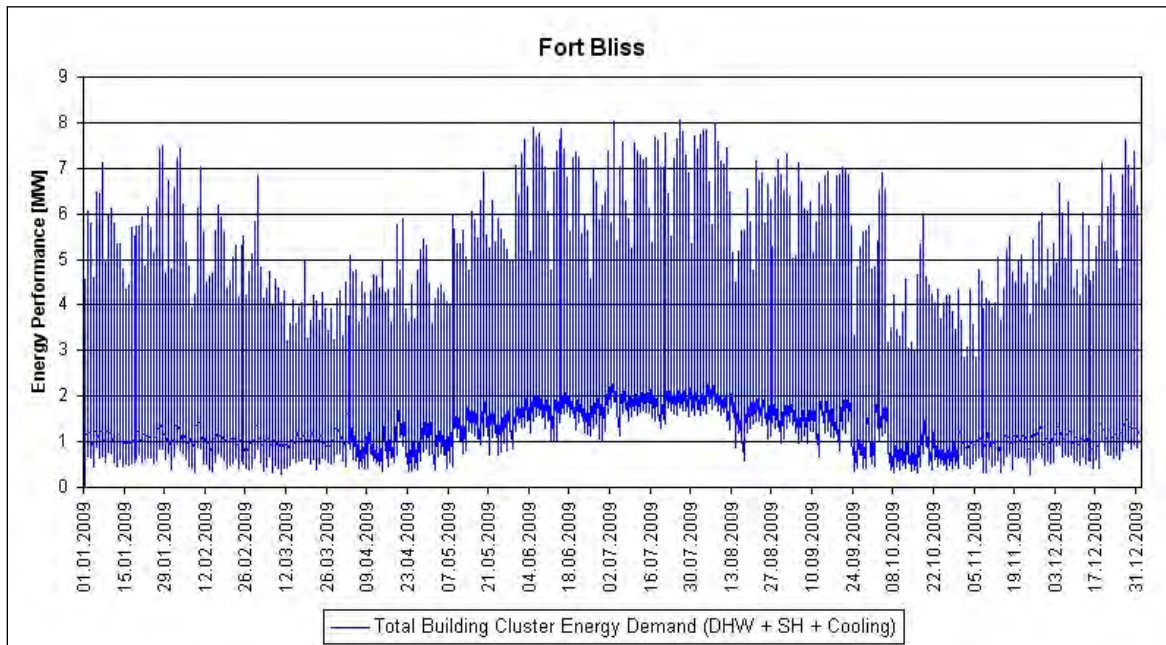
Figure B-8. Energy demand for DHW, space heating and cooling, Fort Bliss solar collector.
