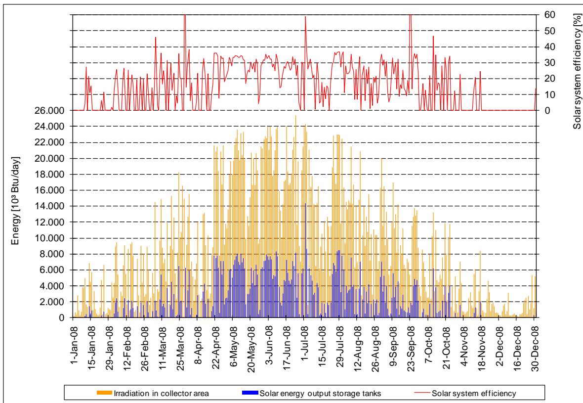
Figure A-60. Irradiation, energy output solar storage tank and efficiency solar system in 2008, daily data solution.
