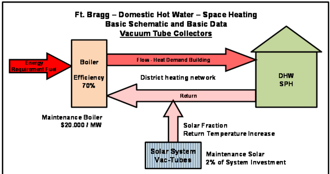
Figure B-35. Basic schematic – Fort Bragg – DHW / SPH – vacuum tube collectors.
