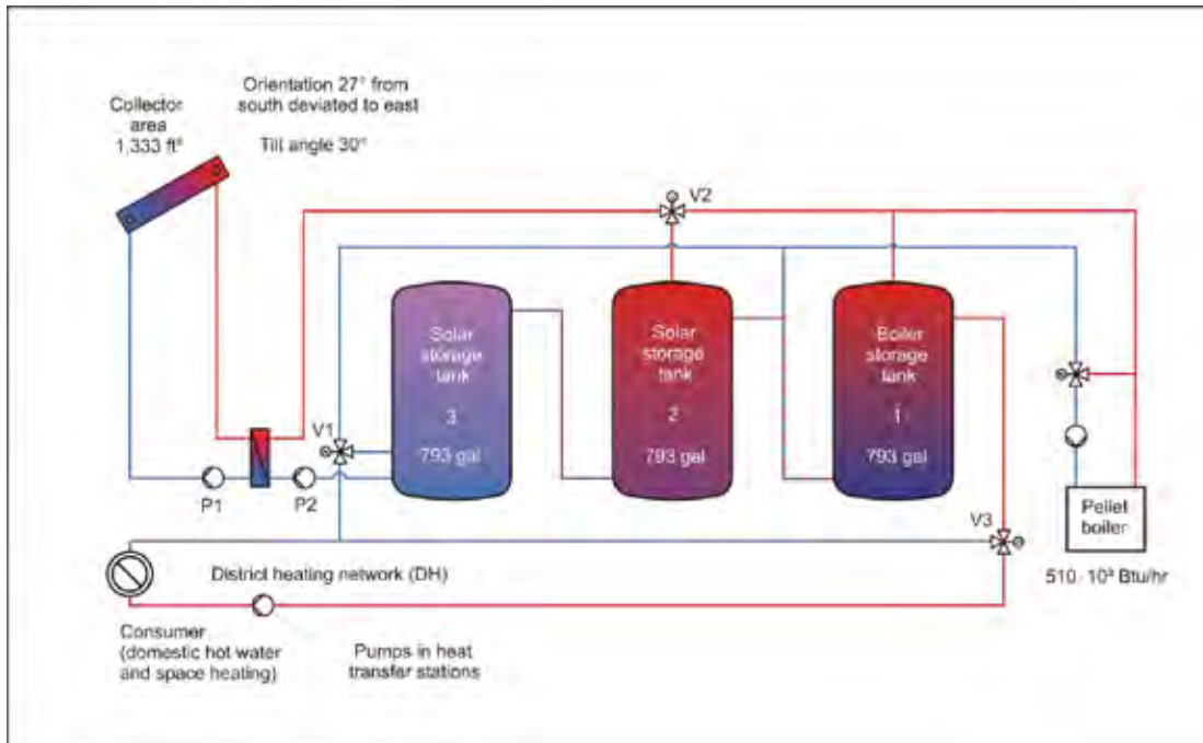
Figure A-75. Highly simplified schematics of the solar system, solar storage tanks arrangement and the integration in the district heating network (DH).
