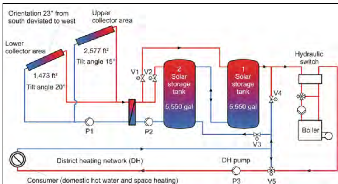
Figure A-65. Highly simplified schematics of the solar system, solar storage tanks arrangement and the integration in the district heating network (DH).
