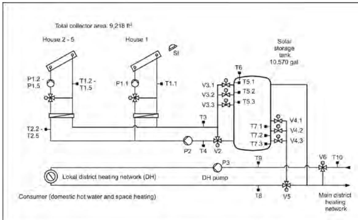
Figure A-61. Highly simplified schematics showing the positioning of the control sensors.
