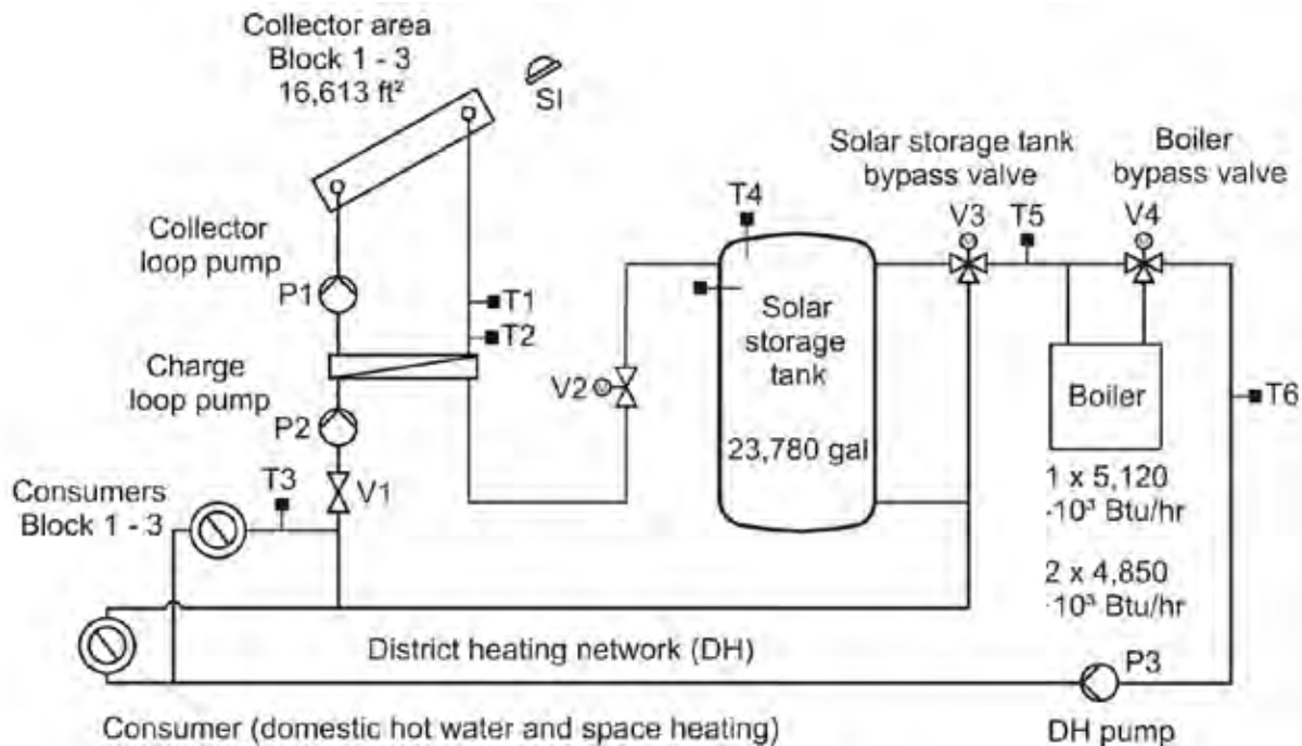
Figure A-84. Highly simplified schematics showing the positioning of the control sensors.
