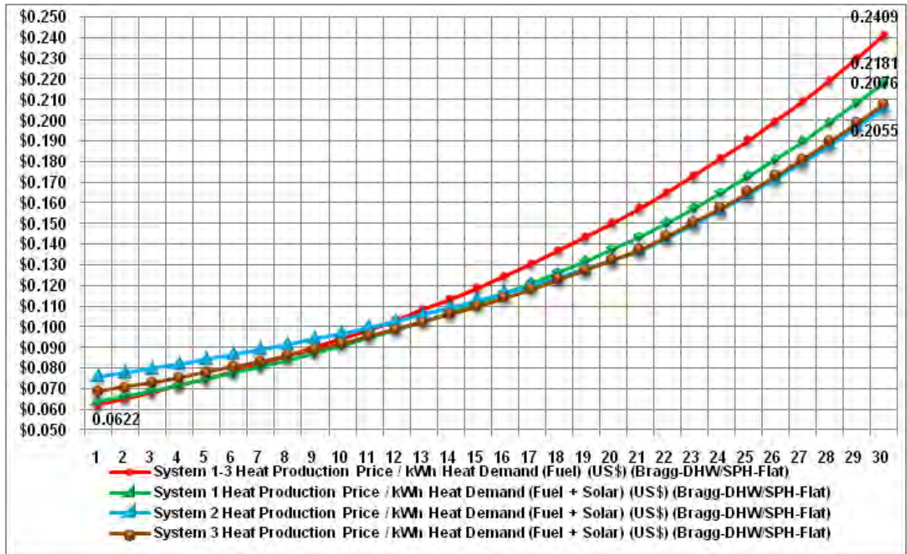
Figure B-41. Energy cost - Fort Bragg – DHW / SPH – flat plate collectors.
