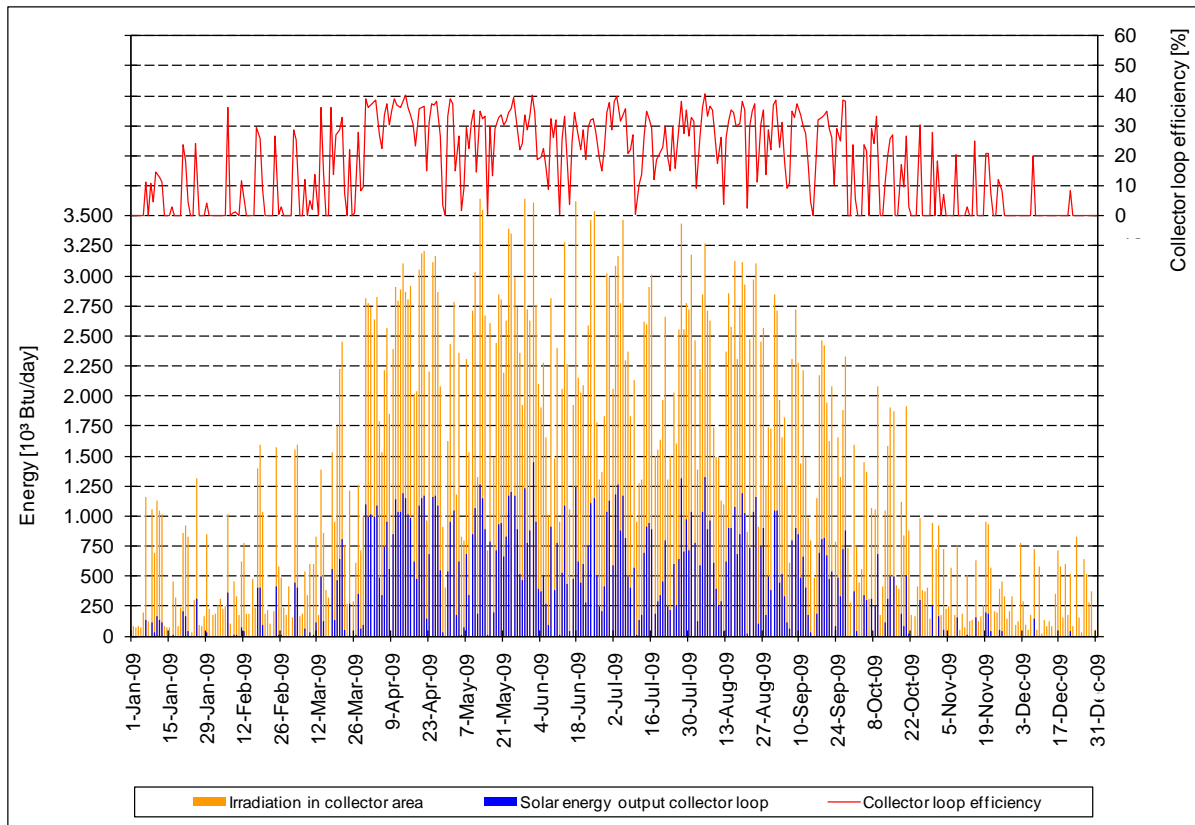
Figure A-76. Irradiation, energy output, and efficiency collector loop in 2009, daily data solution.
