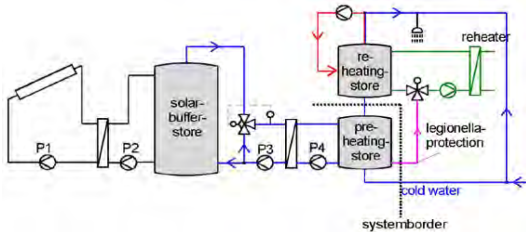
Figure A-38. Solar system for drinking water heating with pre-heating store and thermal disinfection for legionella-protection (no coverage of circulation losses).
