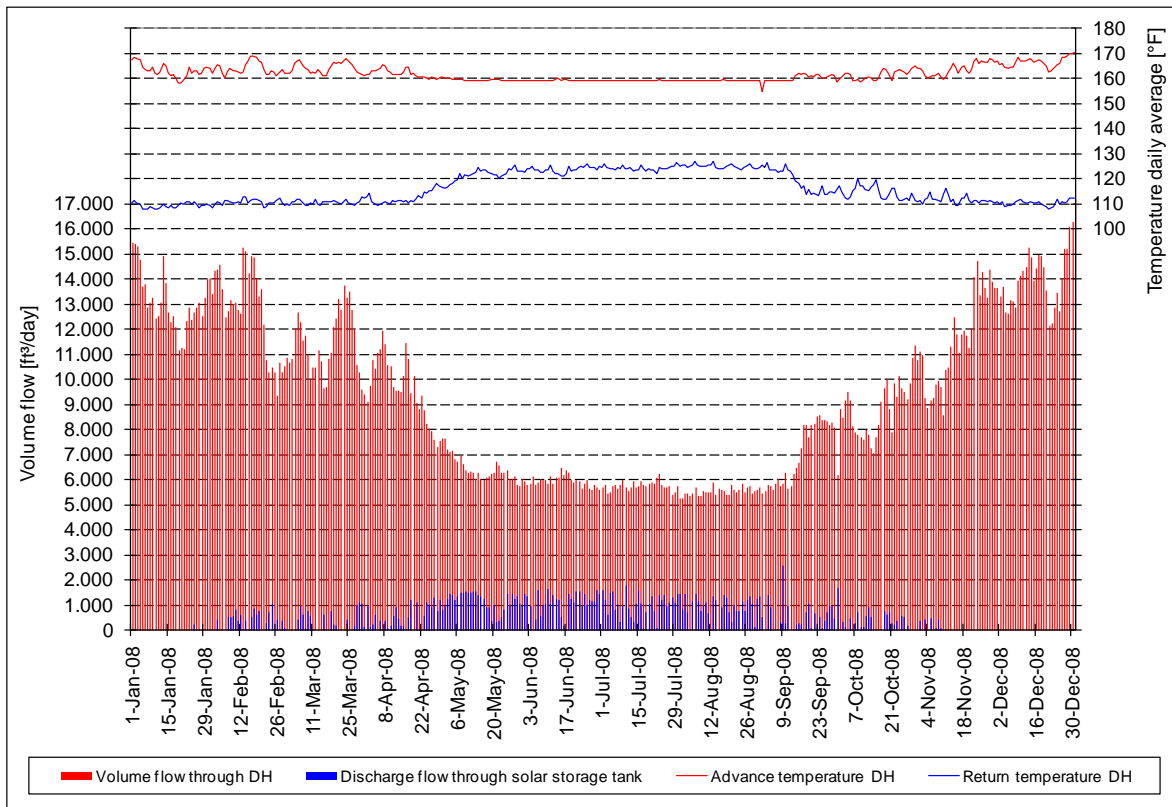
Figure A-72. Volume flow DH, discharge flow through solar storage tanks and temperatures DH.
