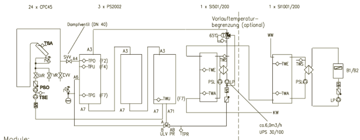
Figure A-113. Schematic view of solar system at Alta Leipziger, Oberunsel, Germany.
