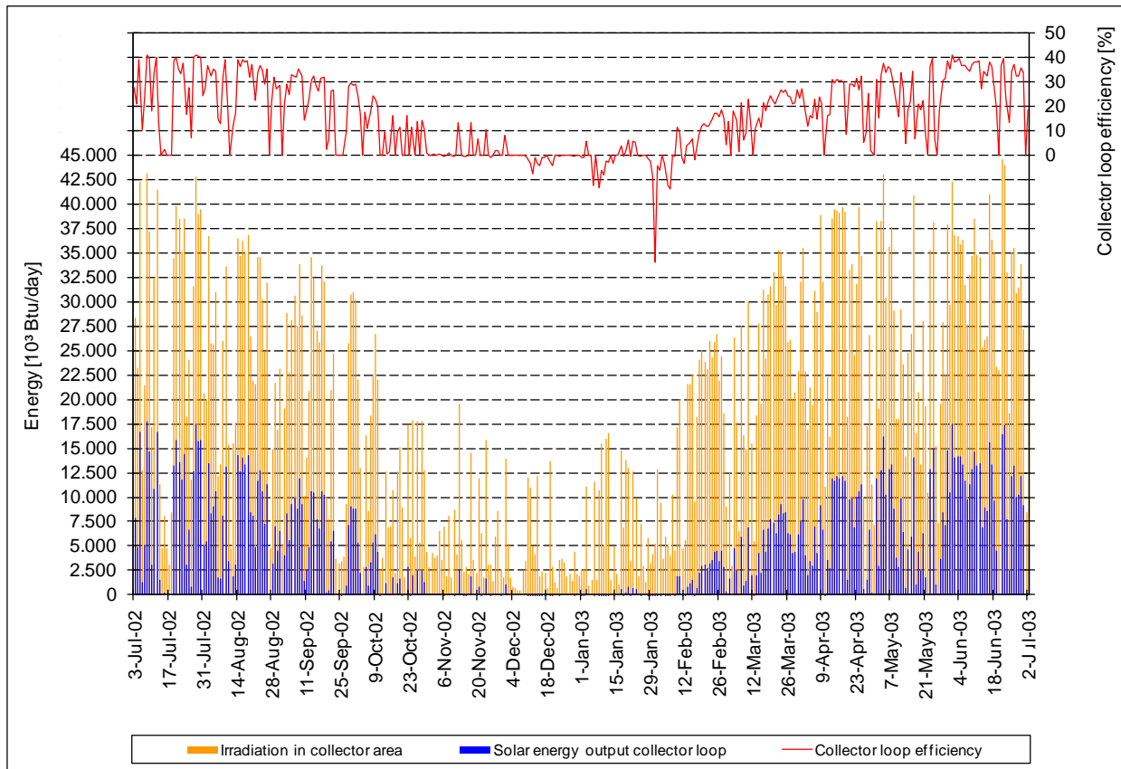
Figure A-83. Irradiation, energy output, and efficiency of collector loop in 2002/2003, daily data solution.
