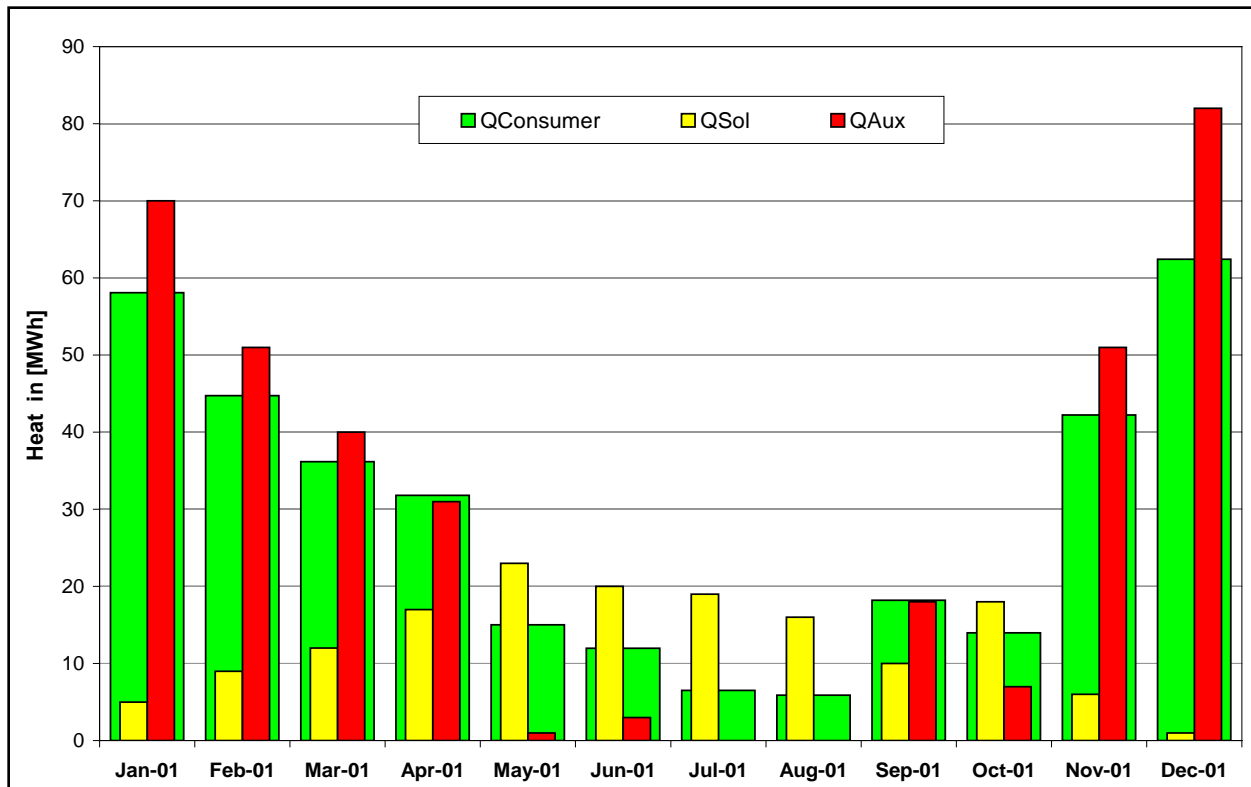
Figure A-4. Heat Balance Gneis-Moos, Salzburg 2001.
