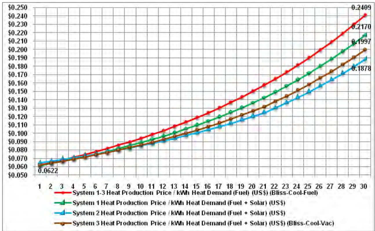
Figure B-22. Energy cost - Fort Bliss – cooling – vacuum tube.
