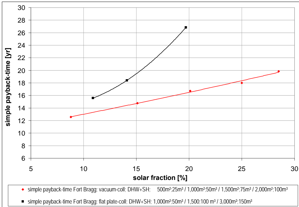
Figure B-34. Simple payback time as a function of solar fraction Fort Bragg, DHW and space heating.
