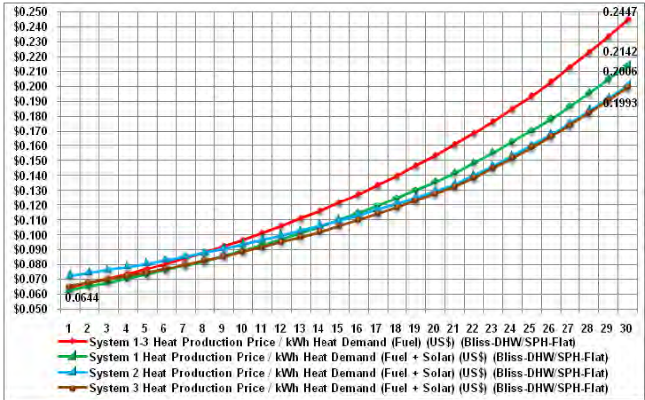
Figure B-31. Energy cost - Fort Bliss - DHW / SPH - flat plate collectors.
