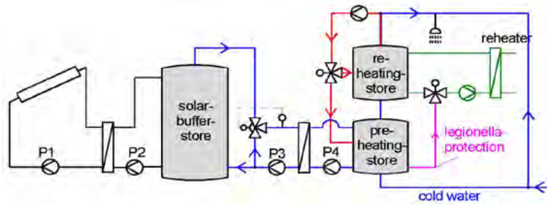
Figure A-39. Solar system for drinking water heating with pre-heating store and thermal disinfection for legionella-protection (with coverage of circulation losses).
