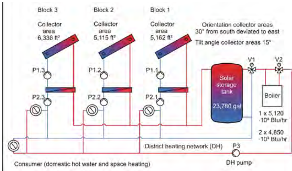
Figure A-82. Highly simplified schematics of the solar system, solar storage tank arrangement and the integration in the district heating network (DH).
