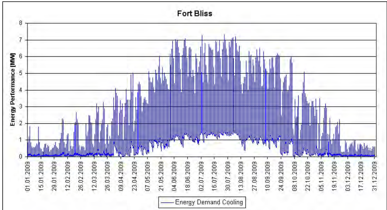
Figure B-5. Energy demand for cooling (Fort Bliss).
