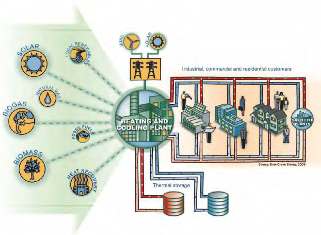
Figure A-104. District Energy St. Paul Integrated Energy Diagram™ .
