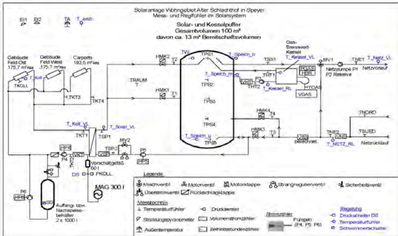
Figure A-45. Piping schematic of the solar system and the connection to district heating net (Speyer “Old Slaughterhouse”).
