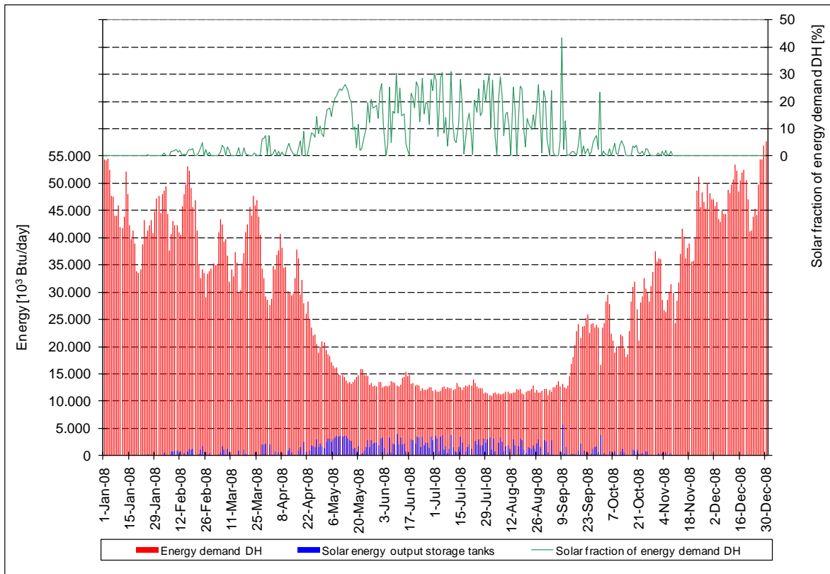
Figure A-71. Energy demand DH, solar energy output solar storage tanks and solar fraction of energy demand DH measured in 2008.
