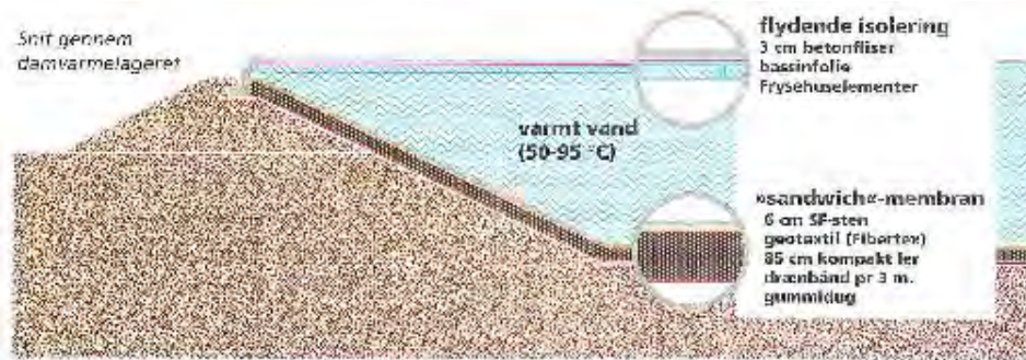
Figure A-31. Cross section of seasonal storage system.
