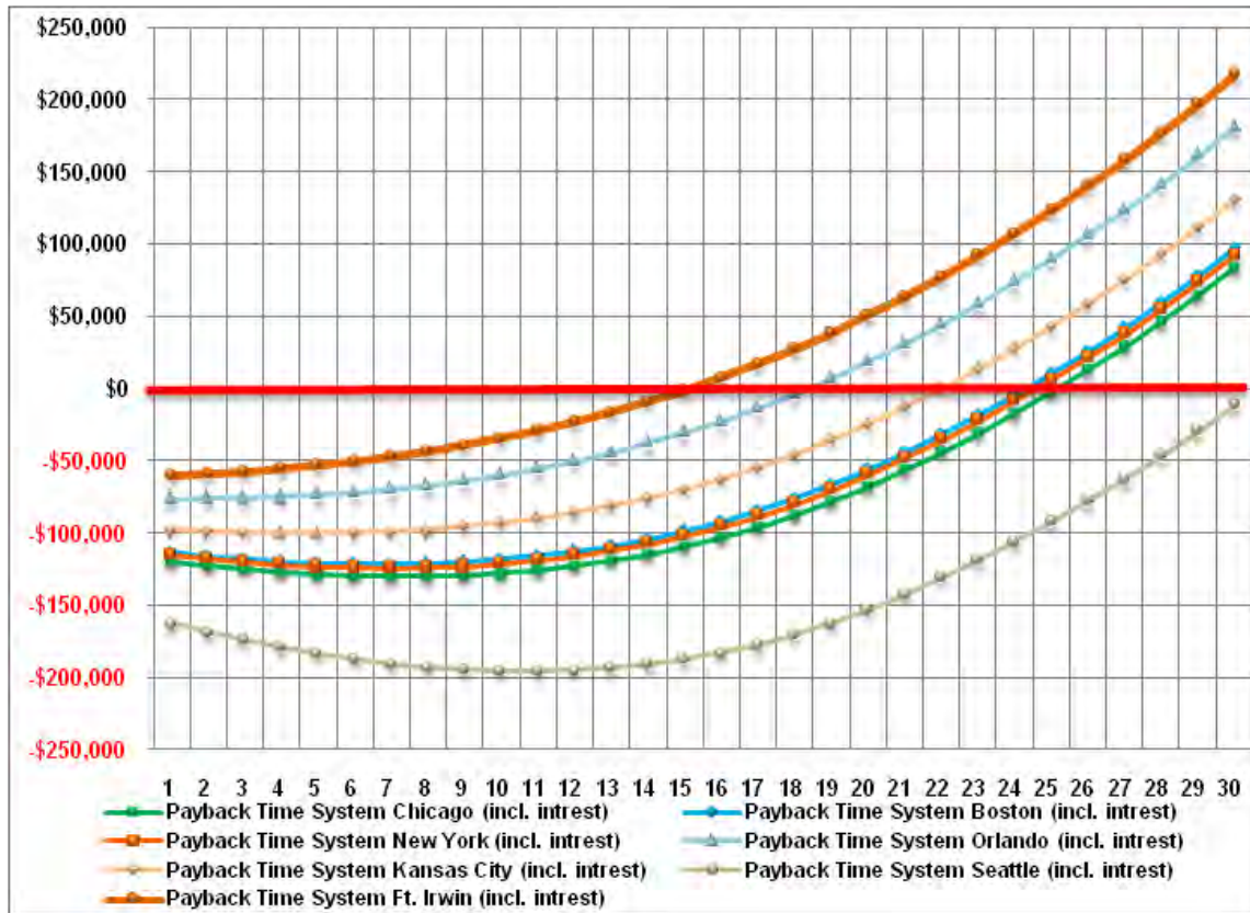
Figure C-4. Comparison of payback time scenario 1 – climate zones.
