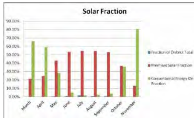
Figure A-100. Solar fraction (2011).
