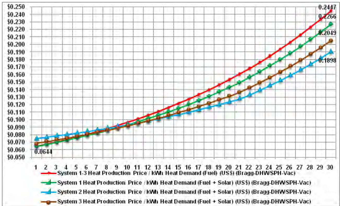
Figure B-37. Energy cost - Fort Bragg – DHW / SPH – vacuum tube collectors.
