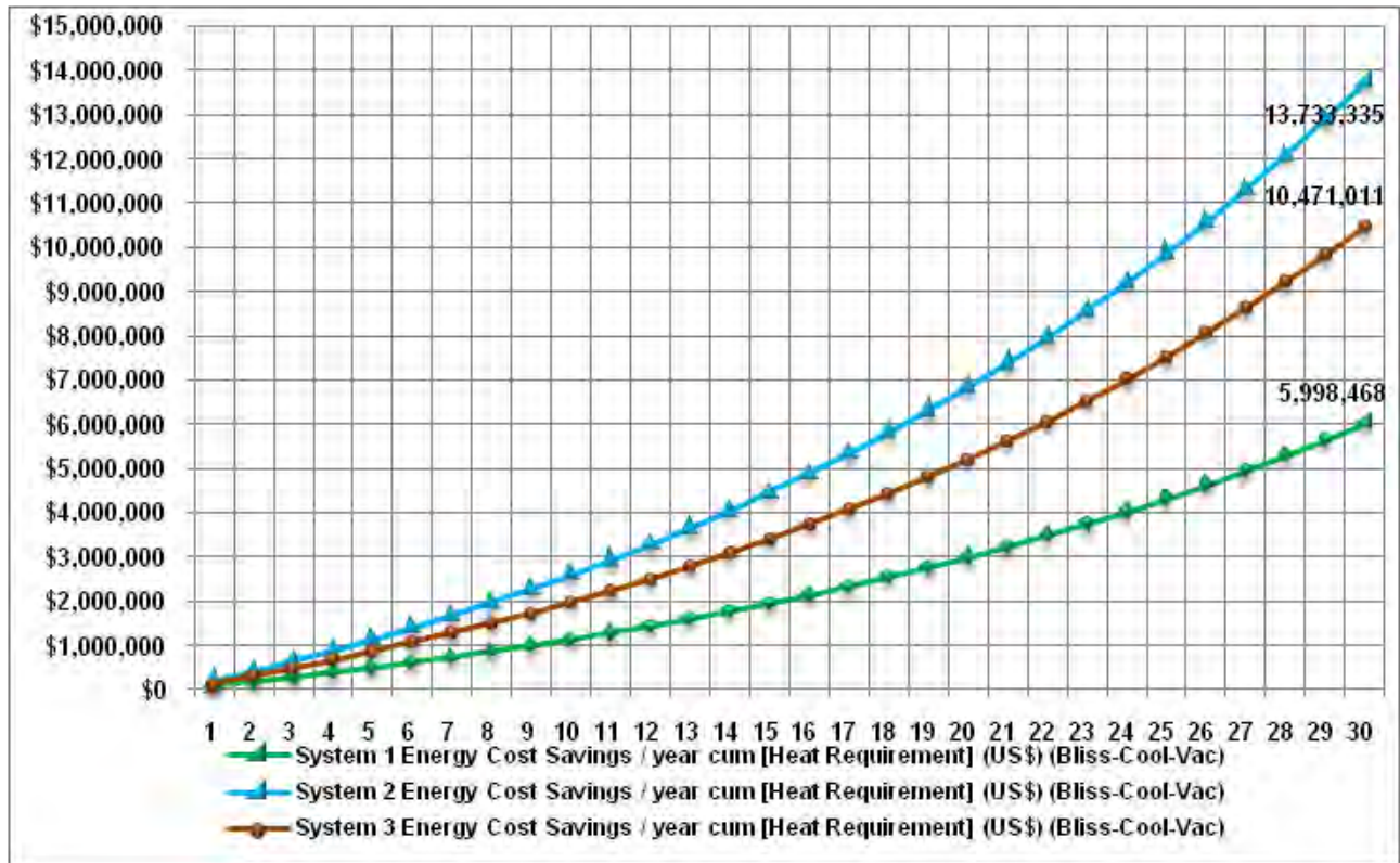
Figure B-23. Energy cost saving / year (cum) – Fort Bliss – cooling – vacuum tube.
