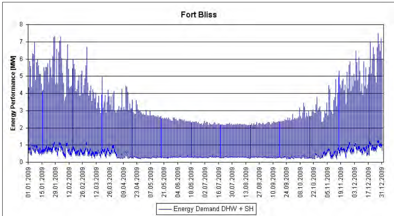
Figure B-11. Energy demand for DHW and space heating, Fort Bliss.
