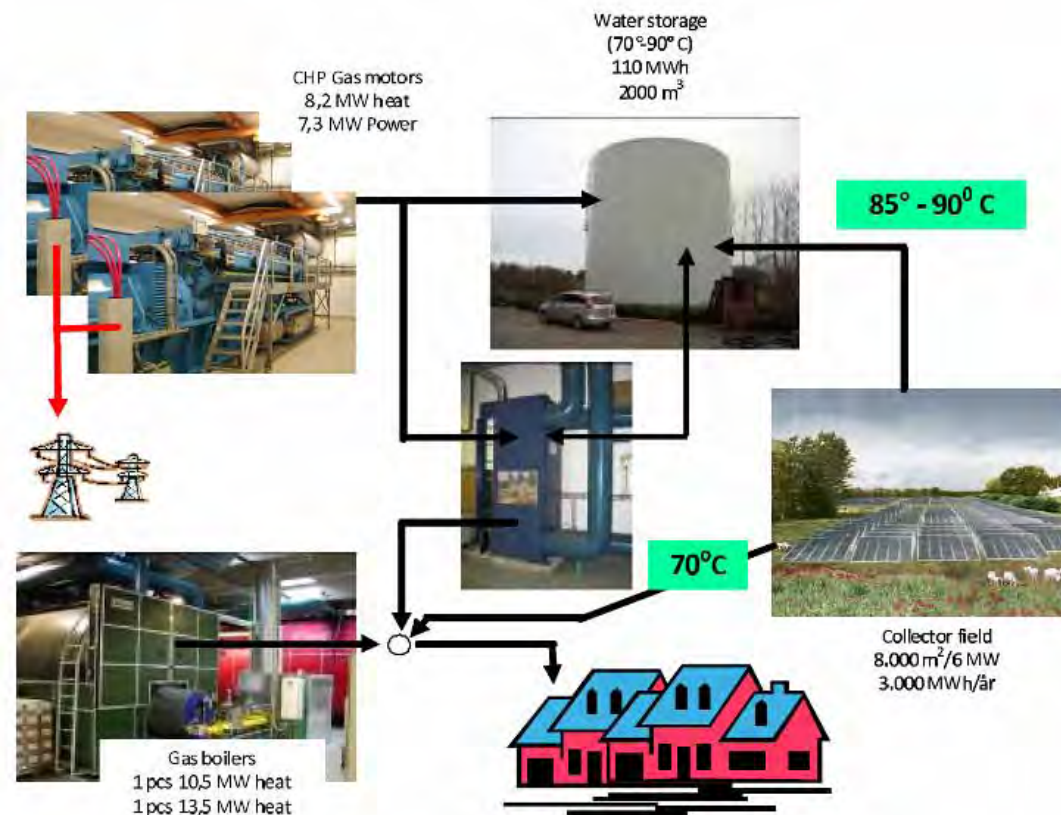
Figure A-34. Overview of the District Heating System of Brædsstrup.
