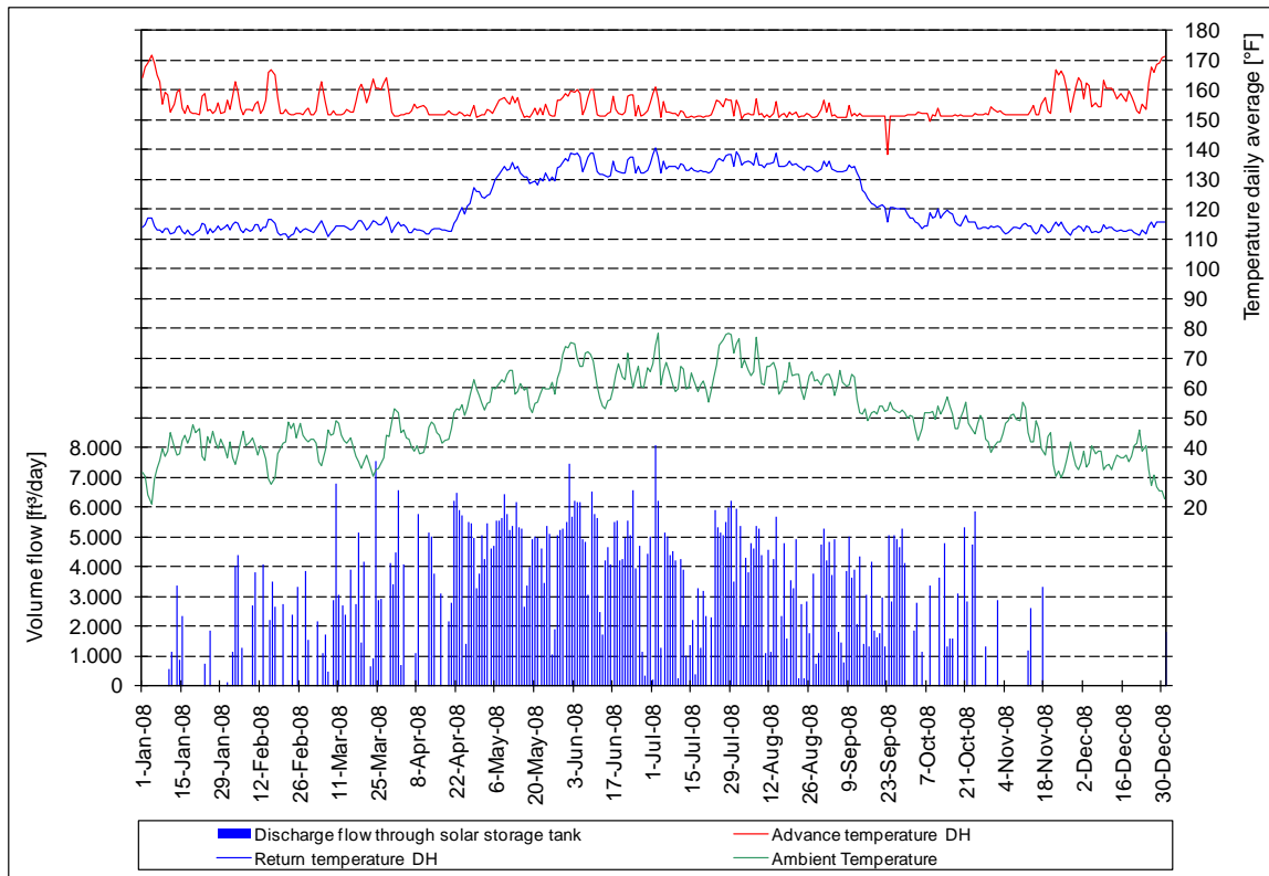
Figure A-62. Discharge flow through solar storage tank and temperatures DH in 2008.
