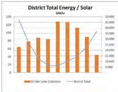
Figure A-99. District energy total solar contribution – RiverCentre installation.
