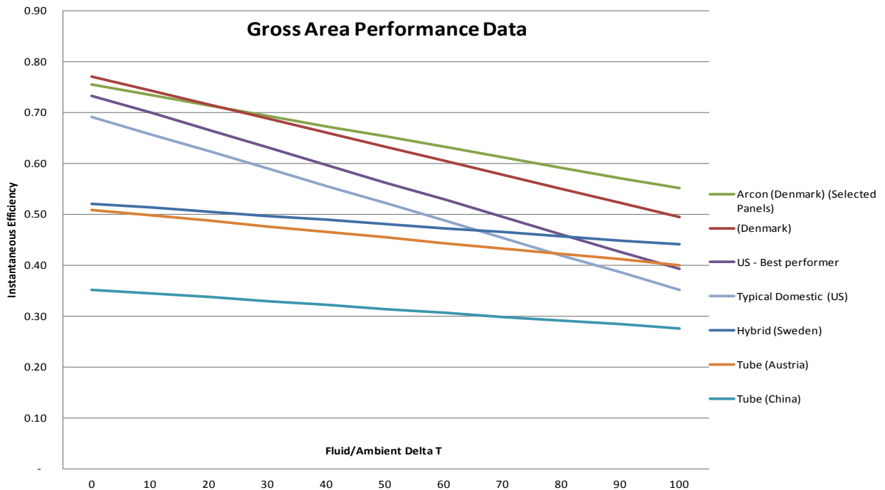
Figure A-92. Gross area performance data for competitive bidders.
