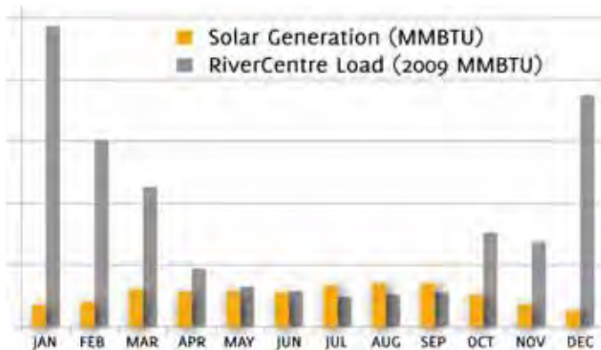
Figure A-97. Energy generation ratio – estimated pre-installation (2010).
