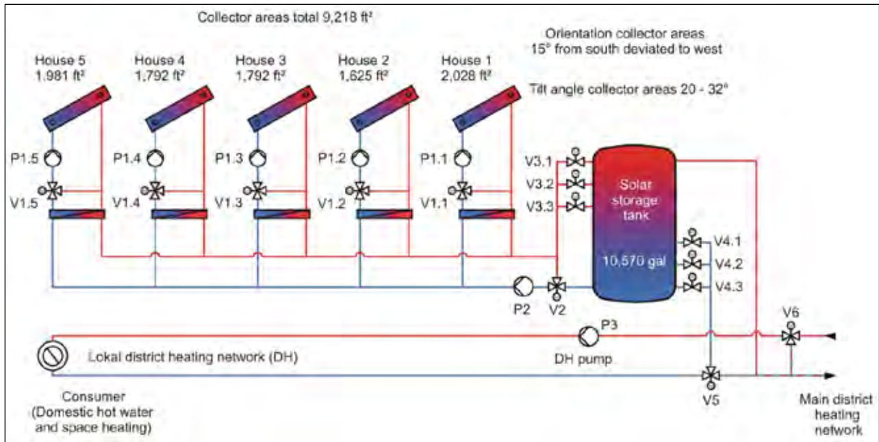
Figure A-56. Highly simplified schematics of the solar system, solar storage tank arrangement, and the integration in the district heating networks.
