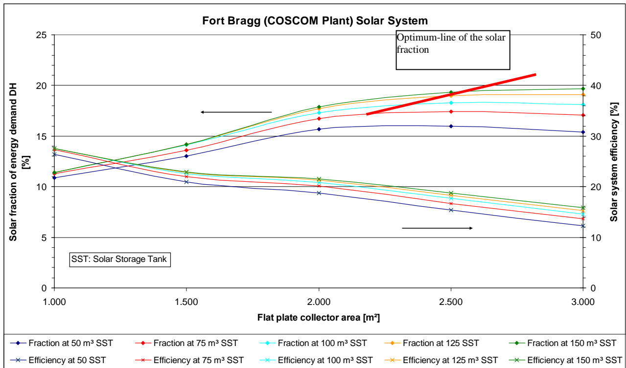
Figure B-19. Solar fraction and solar efficiency depending on flat plate area, Fort Bragg, DHW and space heating.
