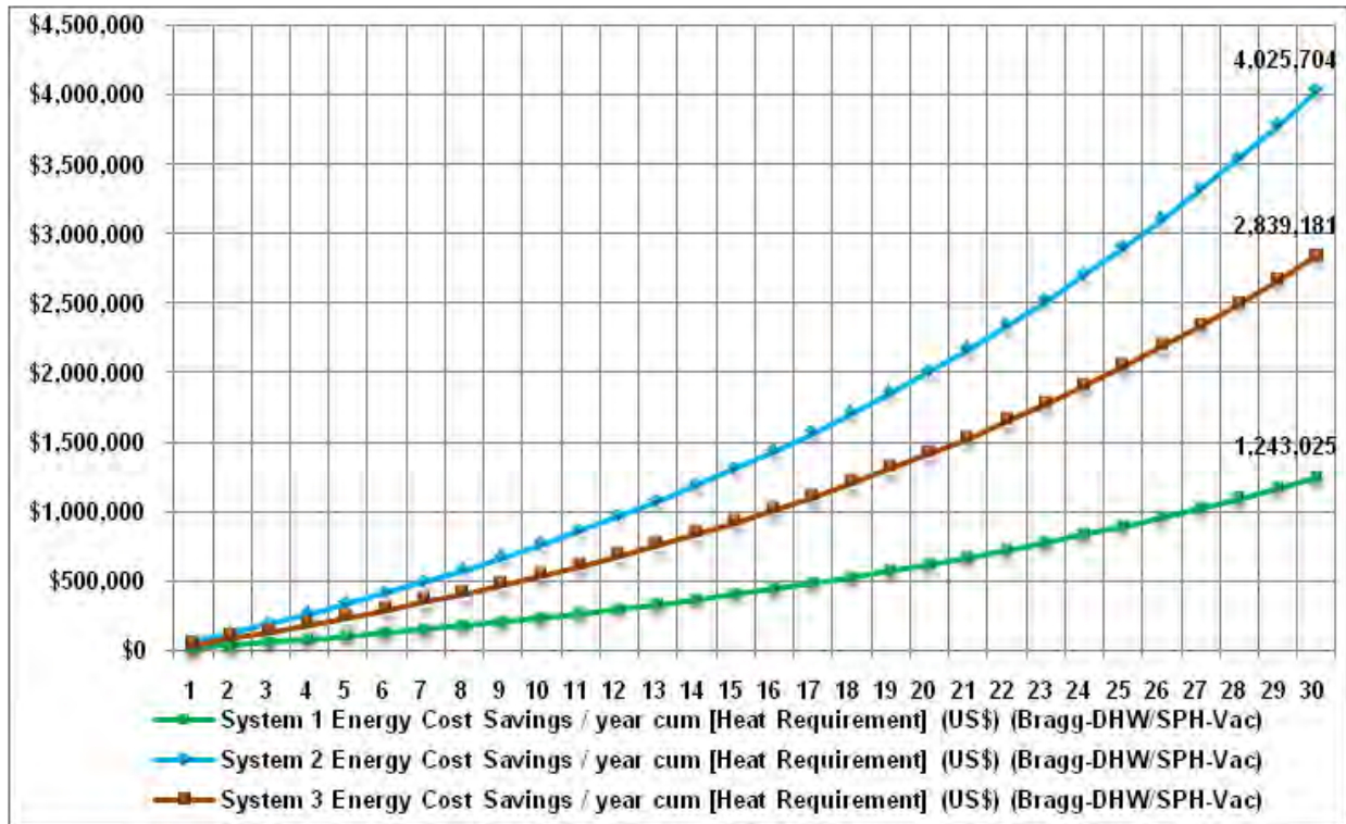
Figure B-38. Energy cost saving / year (cum) – Fort Bragg – DHW / SPH – vacuum tube collectors.
