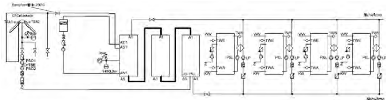
Figure A-117. Schematic view of solar system at Wohnheim Langendamm, Nienburg, Germany.
