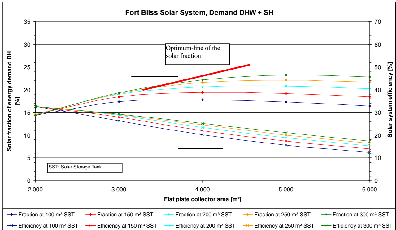
Figure B-13. Solar fraction and solar efficiency depending on flat plate area, Fort Bliss, DHW and space heating.
