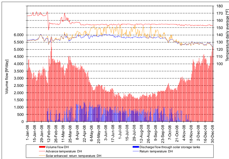
Figure A-53. Volume flow DH, volume flow through solar storage tanks, and temperatures DH.
