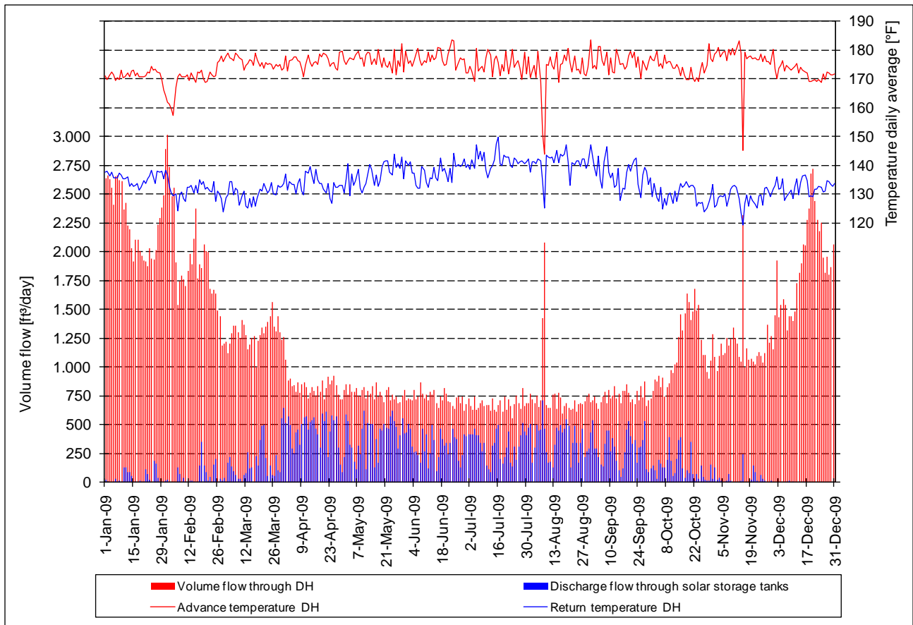
Figure A-79. Volume flow DH, volume flow through solar storage tanks and temperatures DH measured in 2009.
