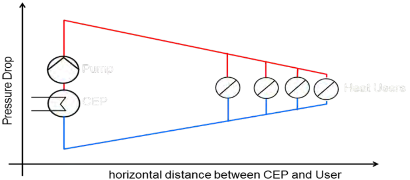
Figure B-2. Typical pressure diagram of a DH system between generation and critical building with the lowest differential pressure.
