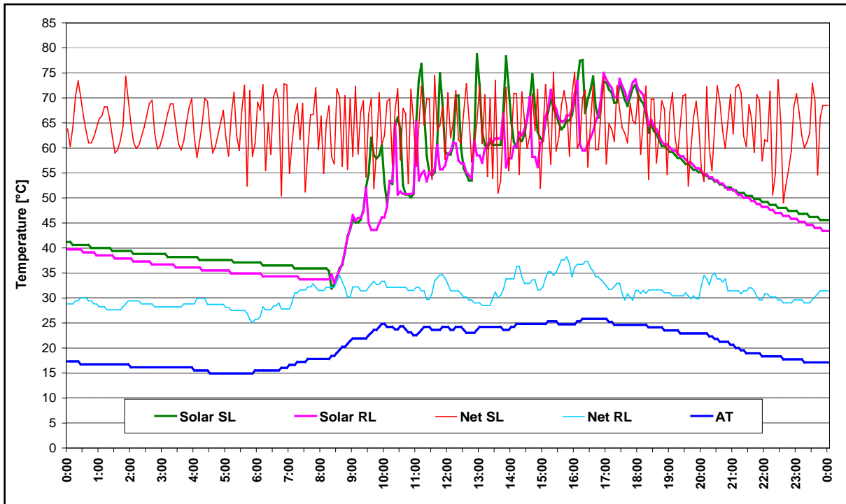
Figure A-9. Temperatures of the solar loop and the distribution grid in July 2 nd 2001, Gneis-Moos.
