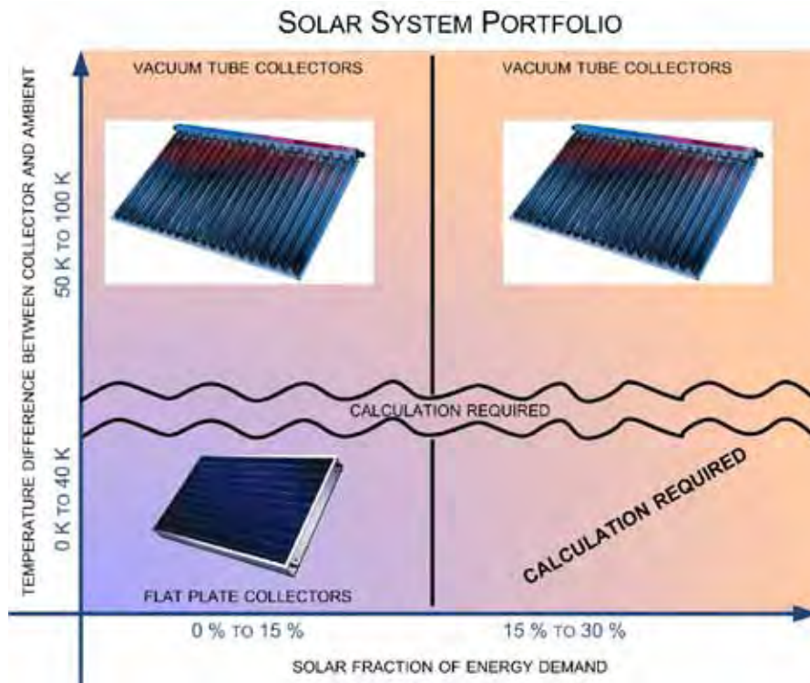
Figure B-43. Solar fraction of energy demand.
