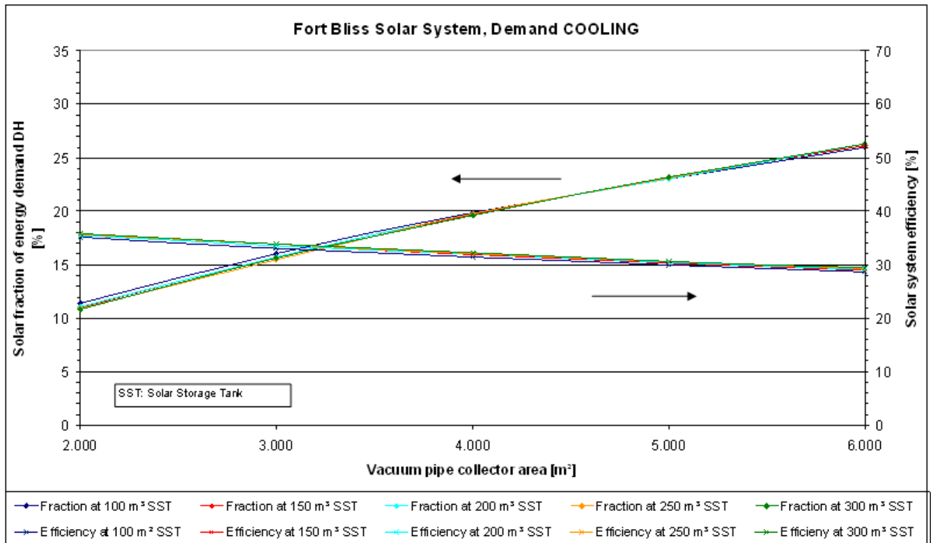
Figure B-7. Solar fraction and solar efficiency depending on vacuum pipe area, Fort Bliss, cooling.
