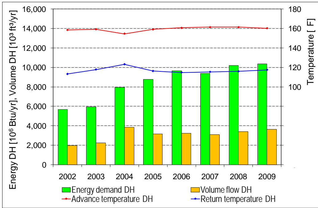
Figure A-68. Energy demand DH, volume flow DH, advance and return temperature DH.
