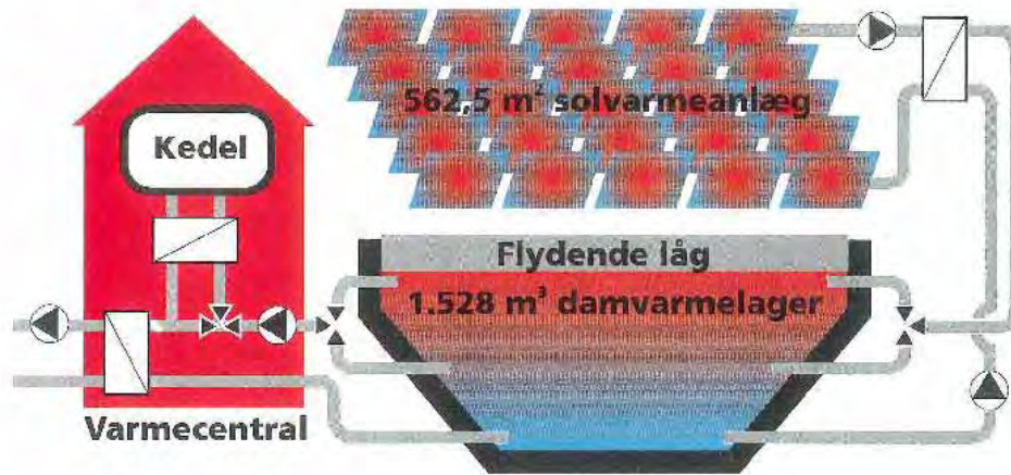
Figure A-29. Diagram of the heating system.
