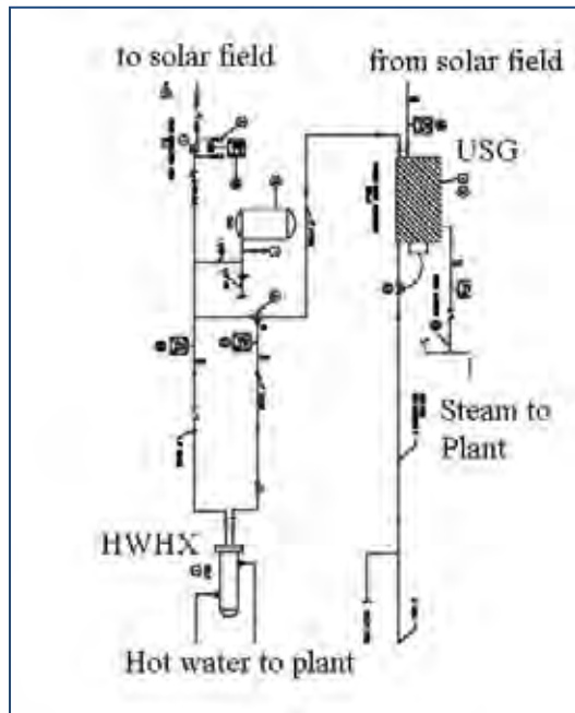
Figure A-127. The balance of systems for the SunChips manufacturing facility includes 285 m of pipe from the solar field to the plant, an unfired steam generator (see Fig. A-109), a heat exchanger, a 25 hp pump, 447 m of pipe running back to the solar field from the plant, and bypass valves and controls.
