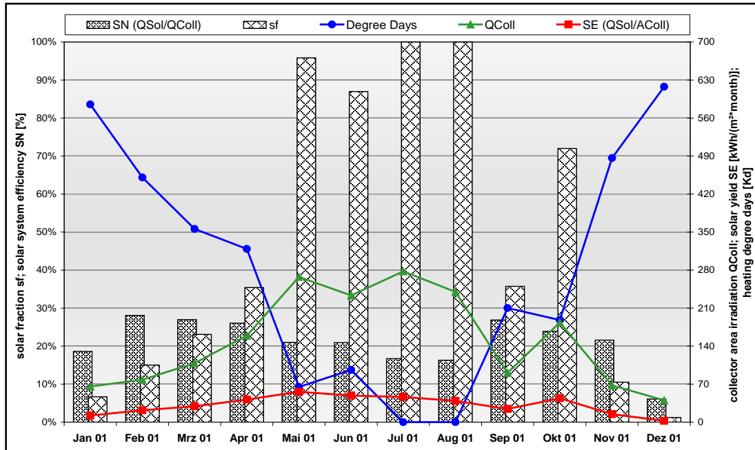
Figure A-3. Solar system performance Gneis-Moos, Salzburg 2001.
