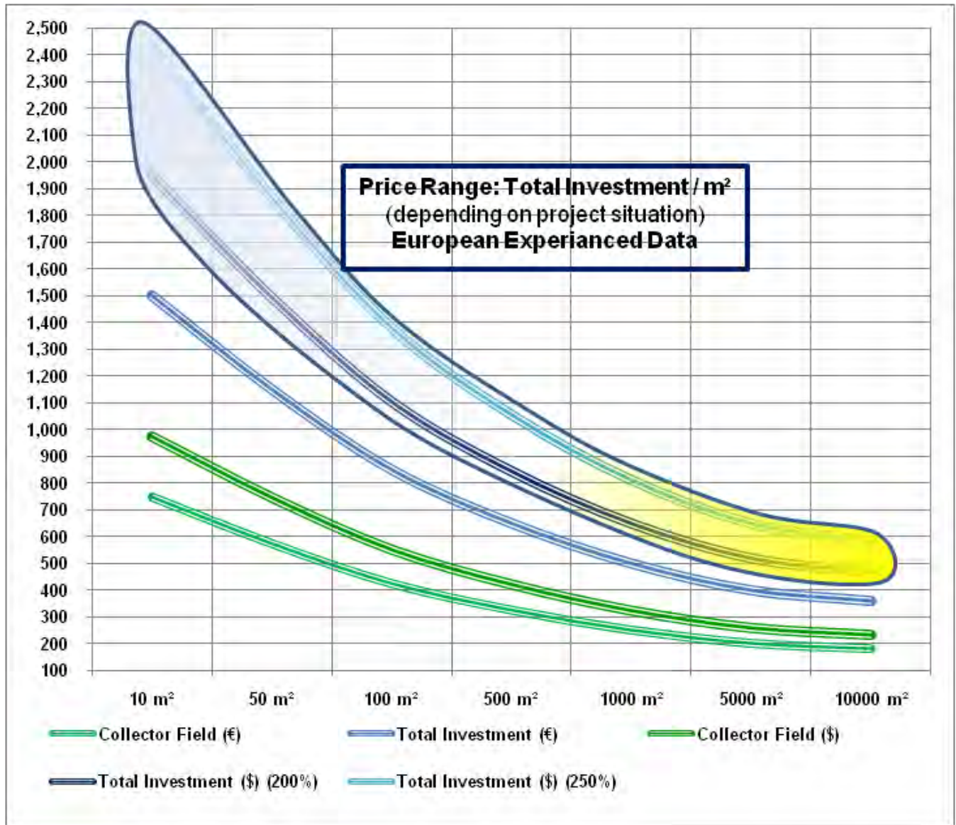
Figure C-1. Price range total investment solar system depending on solar field area.
