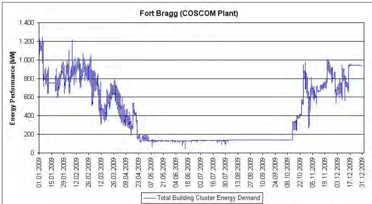
Figure B-14. Metered energy data from COSCOM Plant.
