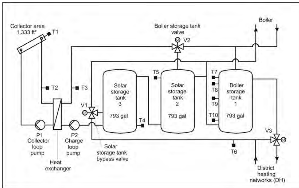
Figure A-77. Highly simplified schematics showing the positioning of the control sensors.
