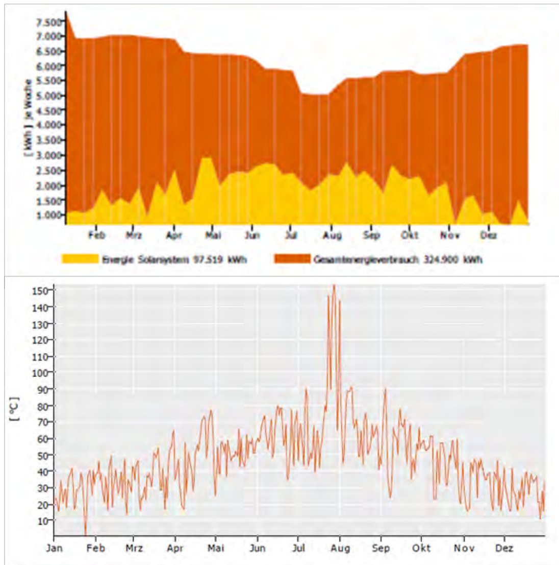
Figure C-3. Solar contribution to energy demand / daily maximum temperature at collector.
