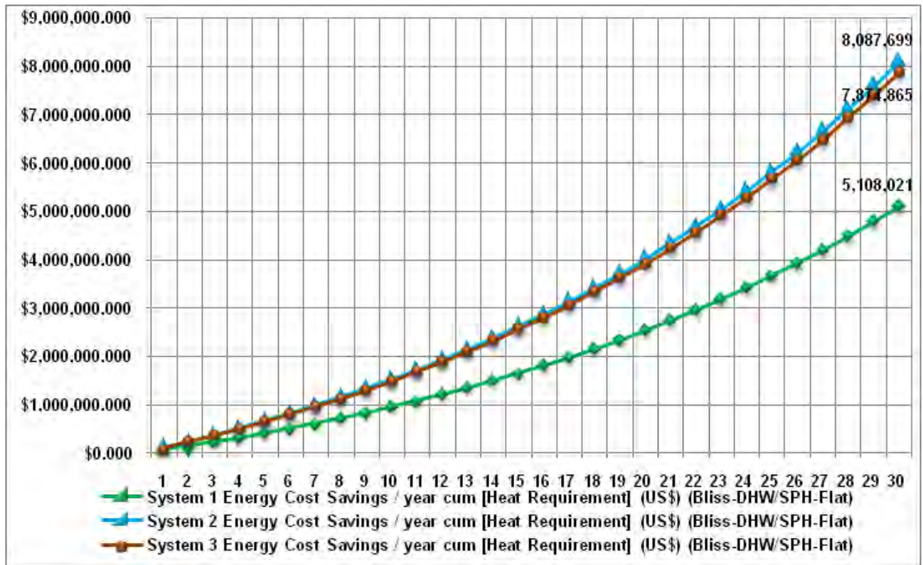
Figure B-32. Energy cost saving / year (cum) - Fort Bliss - DHW / SPH - flat plate collectors.
