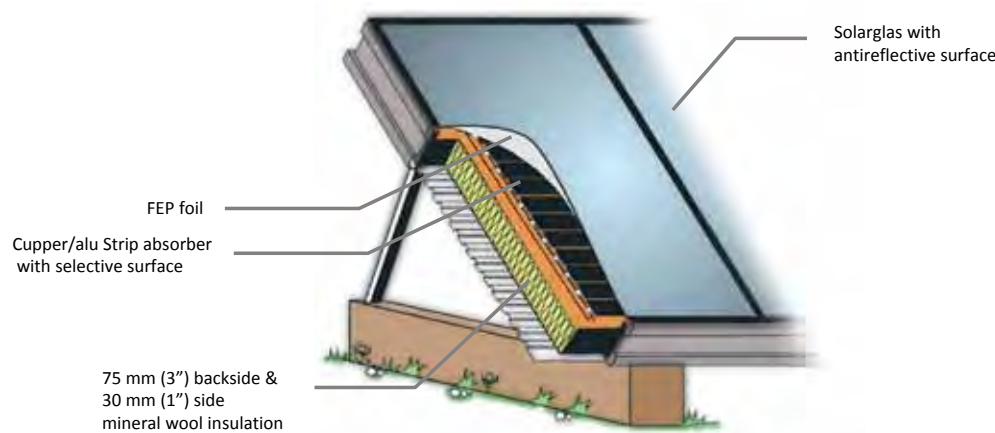
Figure A-35. Cross section of the ARCON HT collector.
