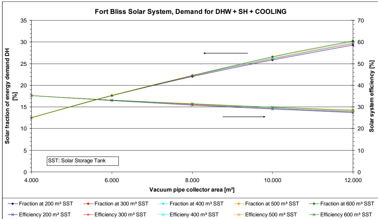
Figure B-10. Solar fraction and solar efficiency depending on vacuum pipe area, Fort Bliss, DHW, space heating and cooling.
