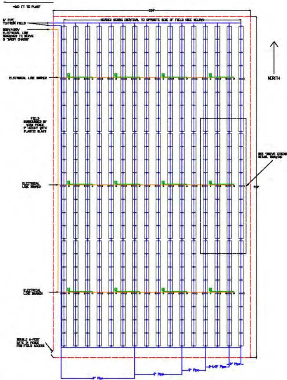
Figure A-126. Schematic of the collector field at the Modesto plant. The field comprises a huge array of concave mirrors. These mirrors track the position of the sun throughout the day, focusing the sun's energy on a black tube that runs along the focus of the array. This black tube is surrounded by a second glass tube that protects it from the air, allowing it to absorb solar energy more effectively. As super heated water passes through the black tube, the solar energy heats it up to 450 °F (232 °C). This water then runs through a boiler system that uses its heat to generate steam, which helps to cook the wheat and heat the cooking oil used in the SunChips® manufacturing process. Cooled water then flows back through the tube to the solar concentrator field to repeat the process.
