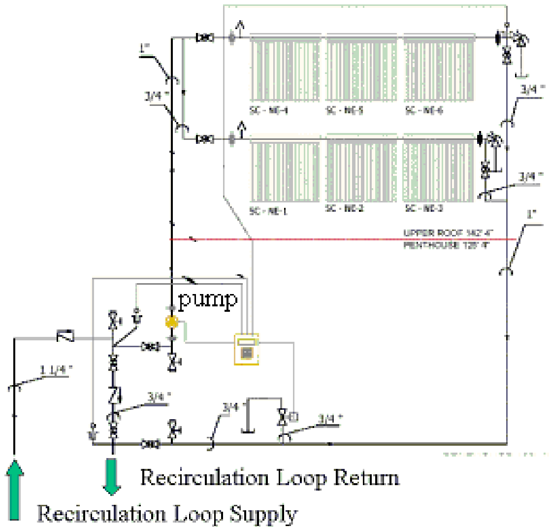
Figure A-107. Schematic diagram of solar water heating system applied to commercial building recirculation loop. This Fig. shows one of two identical systems on the Mid Atlantic Social Security Center.
