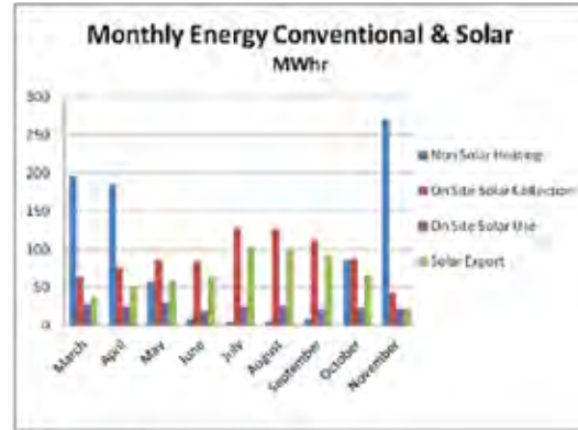
Figure A-102. Monthly energy conventional and solar (2011).
