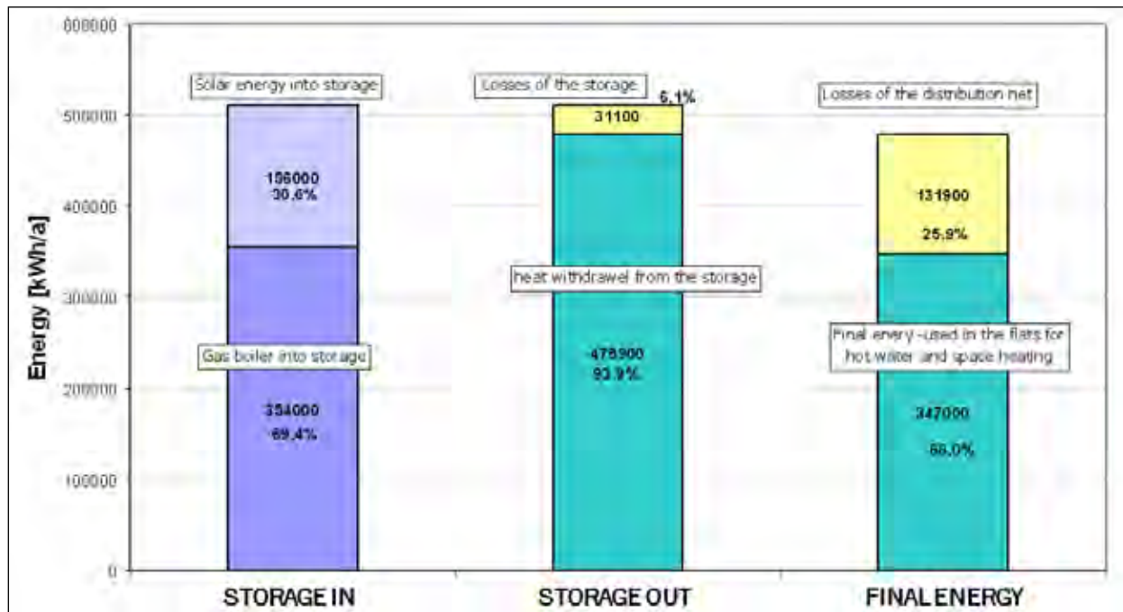
Figure A-5. Energy Balance including system losses Gneis-Moos, Salzburg 2001.
