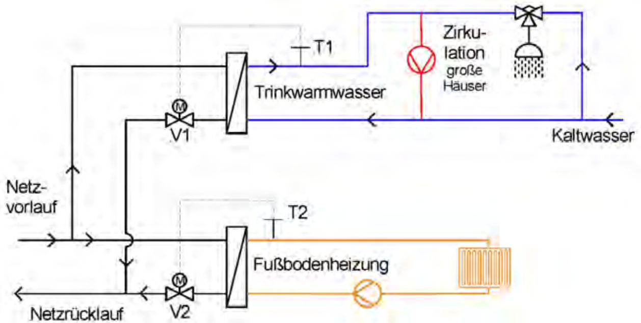
Figure A-44. Piping schematic of heat transfer stations in family houses (District heating Speyer “Old Slaughterhouse”).
