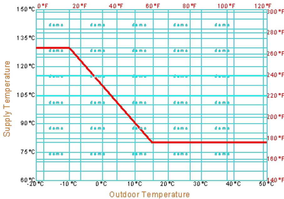
Figure B-1. Relationship between supply temperature and outdoor temperature.
