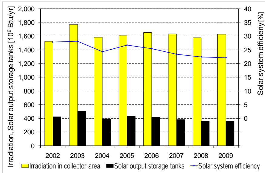
Figure A-66. Irradiation in collector area, solar energy output from solar storage tanks and solar system efficiency.
