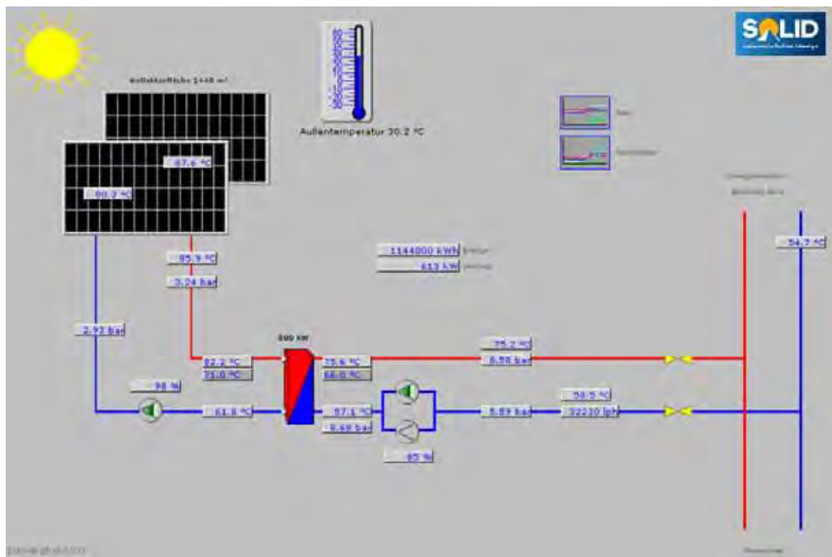
Figure A-18. Block diagram of the centralized collector array connected to the district heating network, UPC arena, Graz-Liebenau, Styria.
