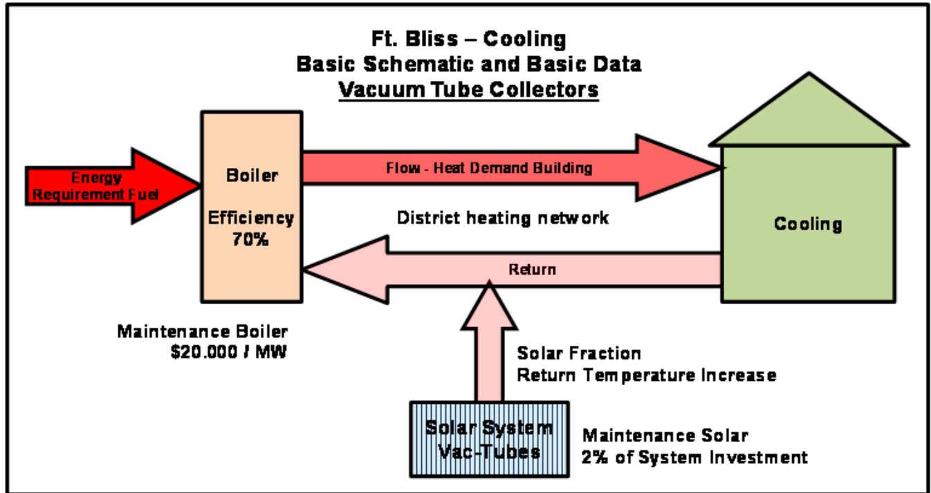
Figure B-20. Basic schematic – Fort Bliss – vacuum tube collectors.
