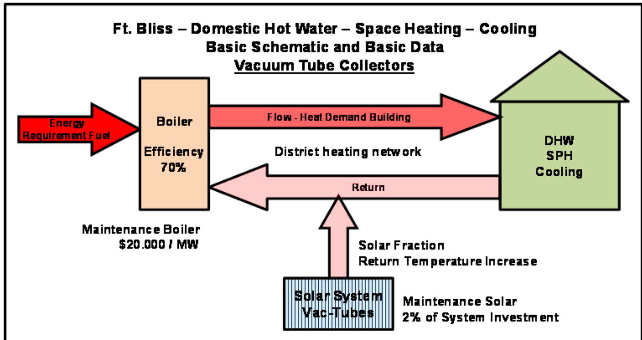
Figure B-24. Basic schematic – Fort Bliss – DHW / SPH / cooling – vacuum tube collectors.
