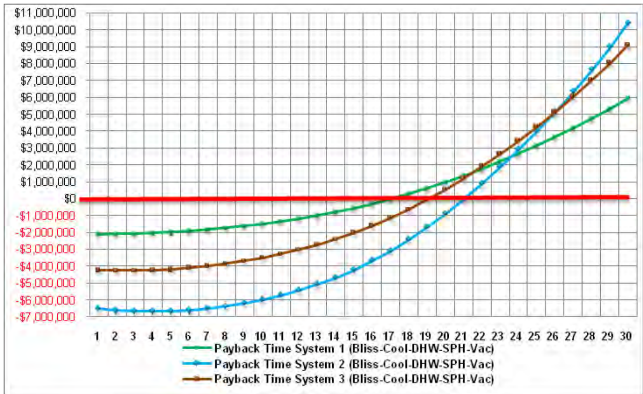
Figure B-25. Payback time - Fort Bliss – DHW / SPH / cooling – vacuum tube collectors.
