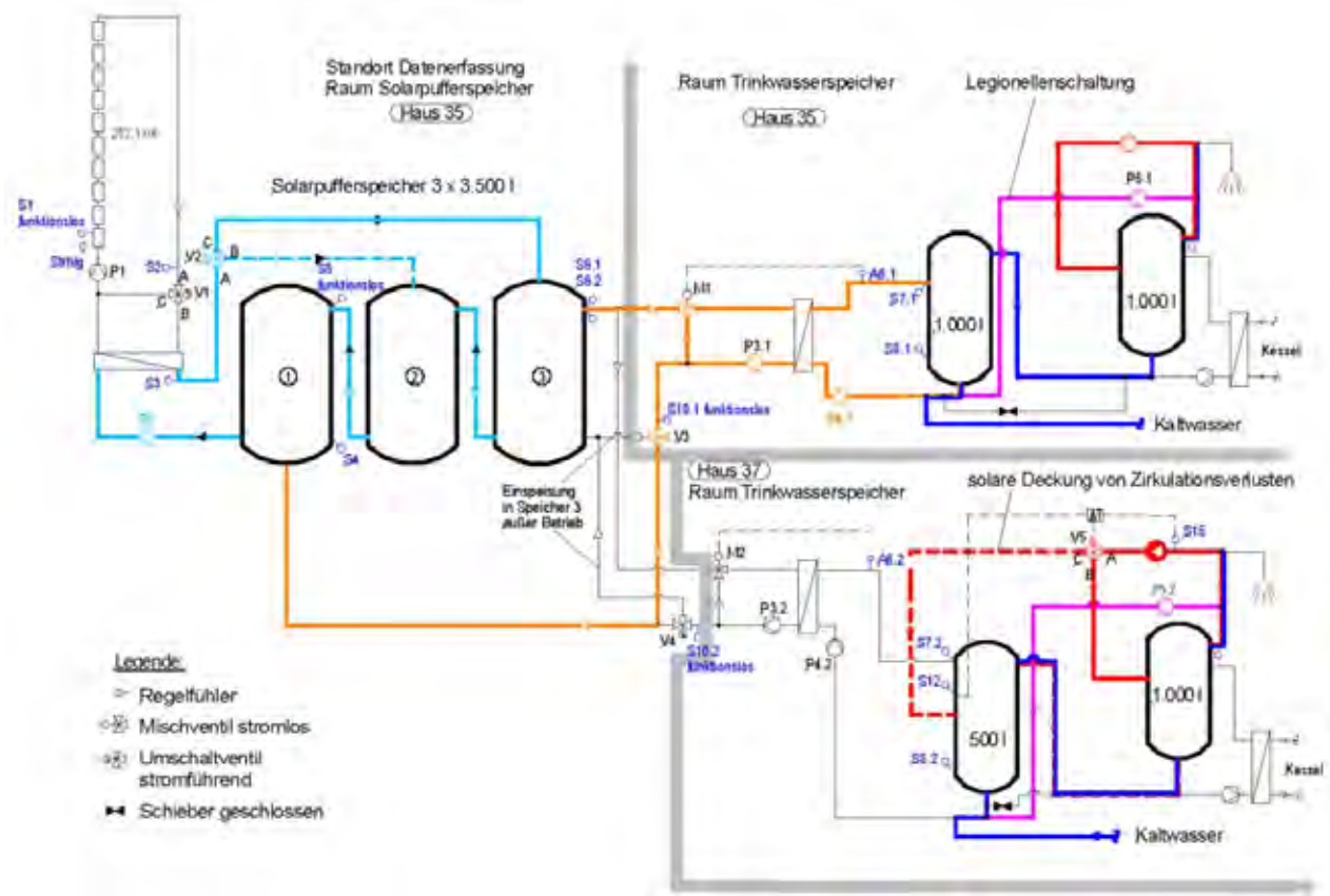
Figure A-40. Piping schematic of the solar system (Apartment House Frankfurt).
