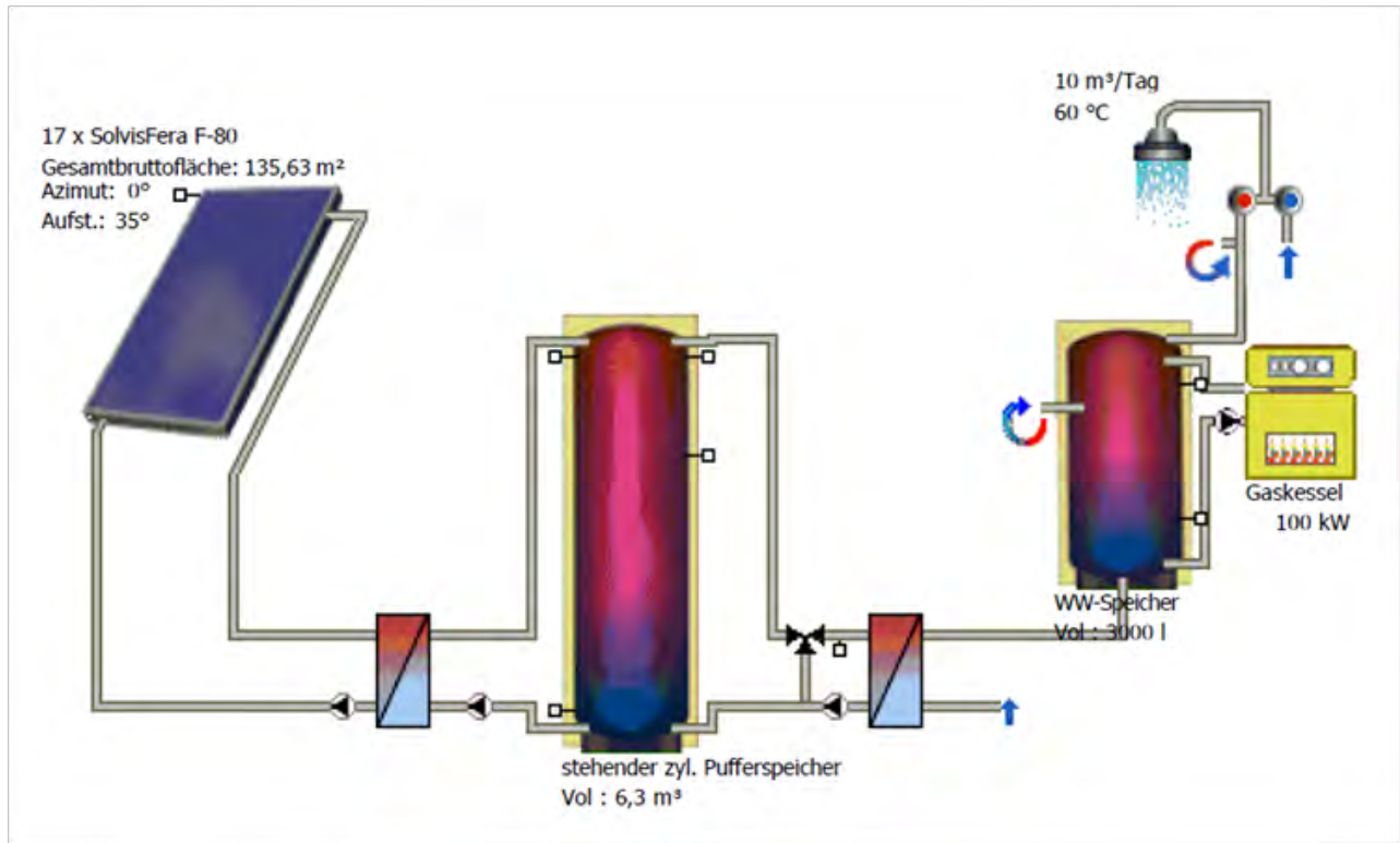
Figure C-2. Schematics of solar system – comparison.
