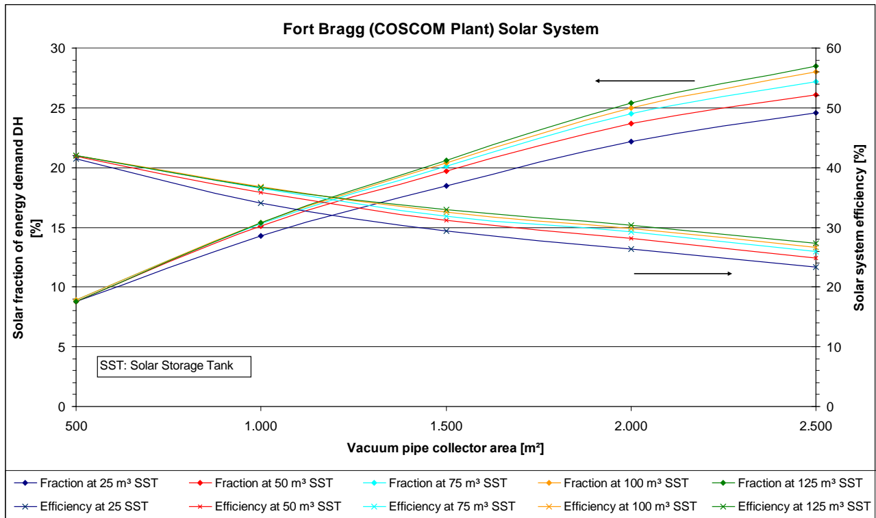
Figure B-16. Solar fraction and solar efficiency depending on vacuum pipe area, Fort Bragg, DHW and space heating.
