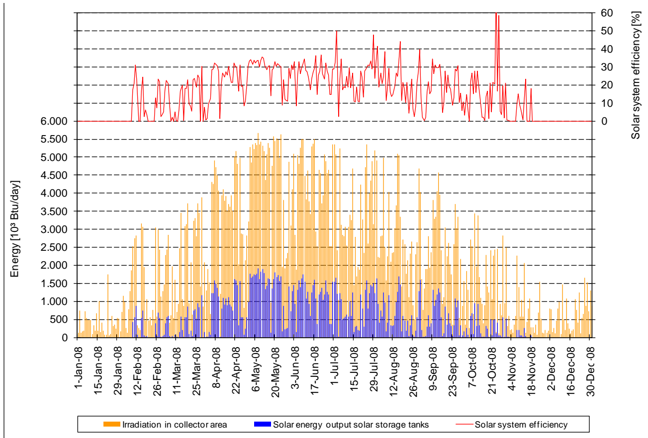
Figure A-50. Irradiation, energy output, and efficiency solar system in 2008, daily data solution.
