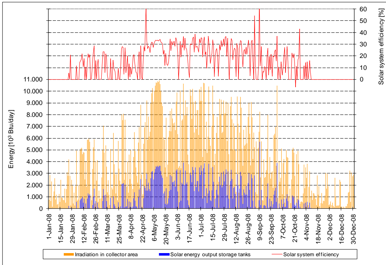
Figure A-69. Irradiation in collector area, solar energy output from solar storage tanks, and solar system efficiency in 2008, daily data solution.
