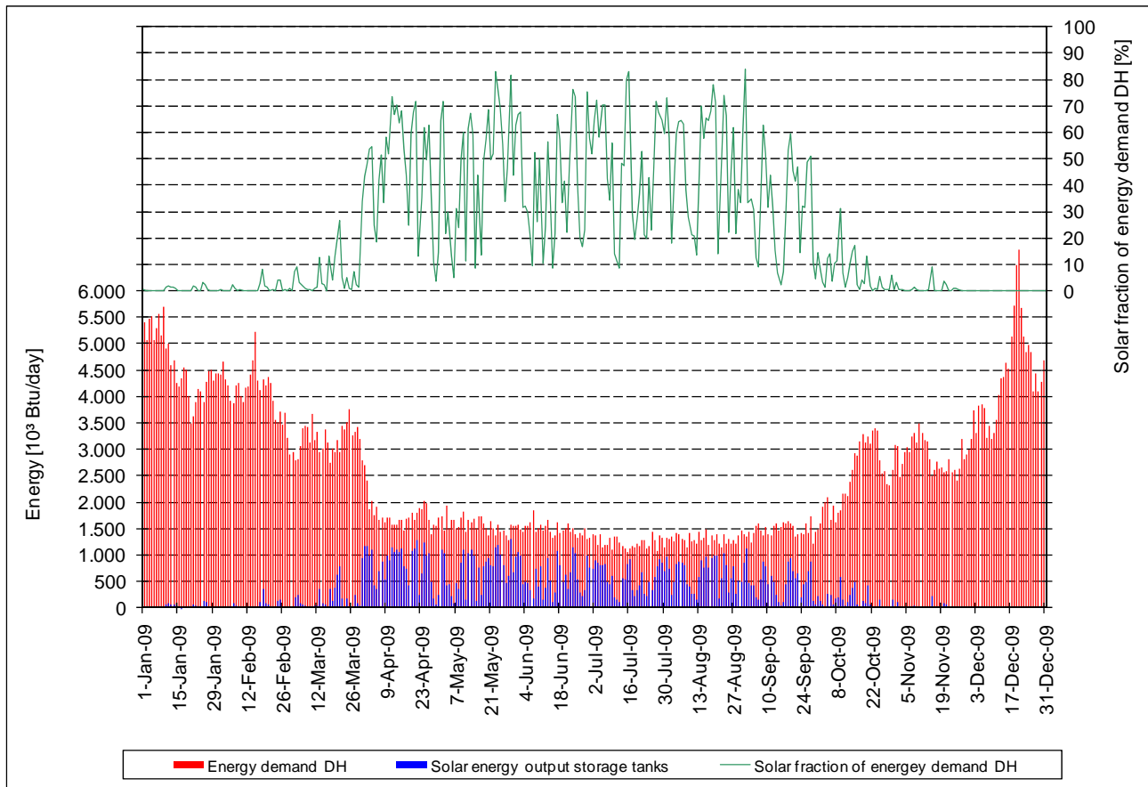
Figure A-78. Energy demand DH, energy output solar system and solar fraction of total energy demand DH measured in 2009.
