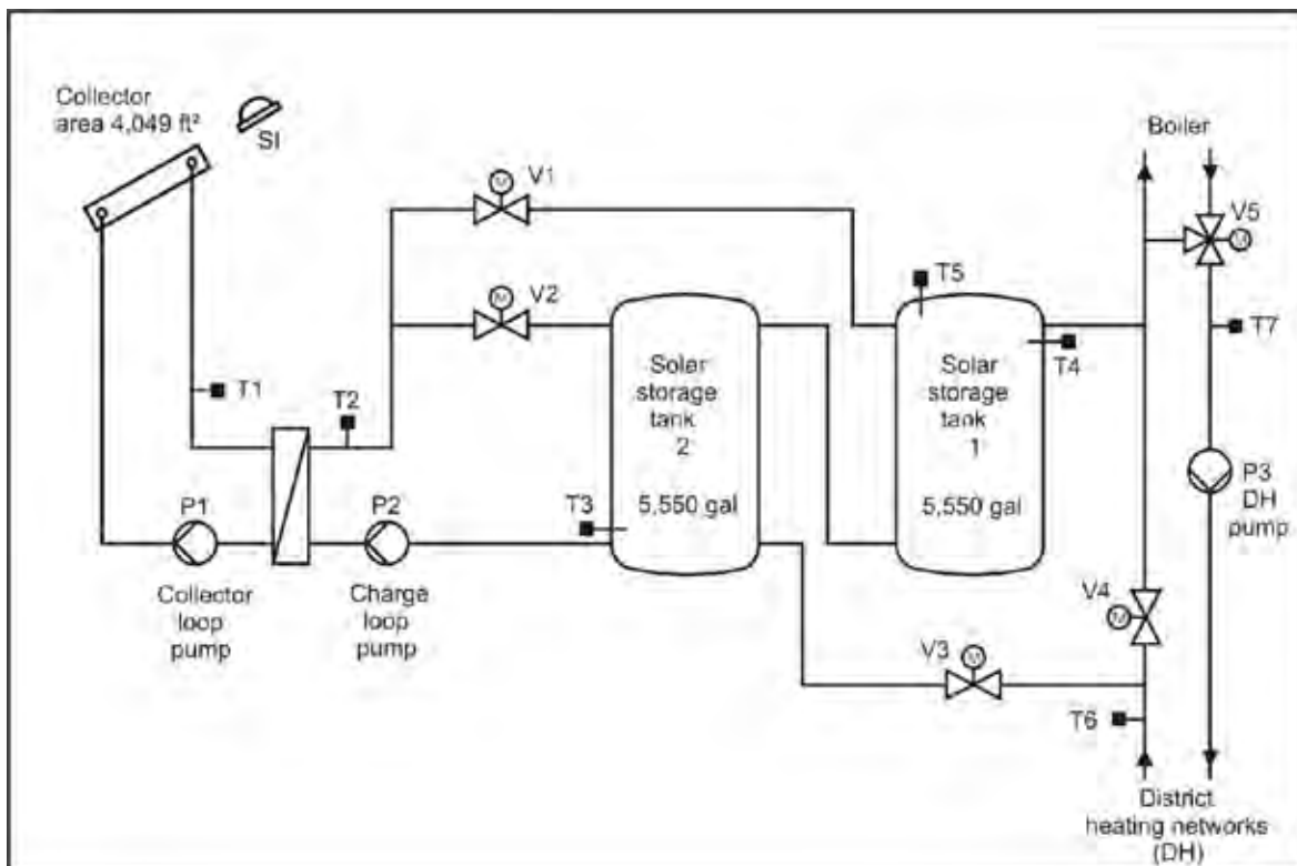
Figure A-70. Highly simplified schematic showing the positioning of the control sensors
