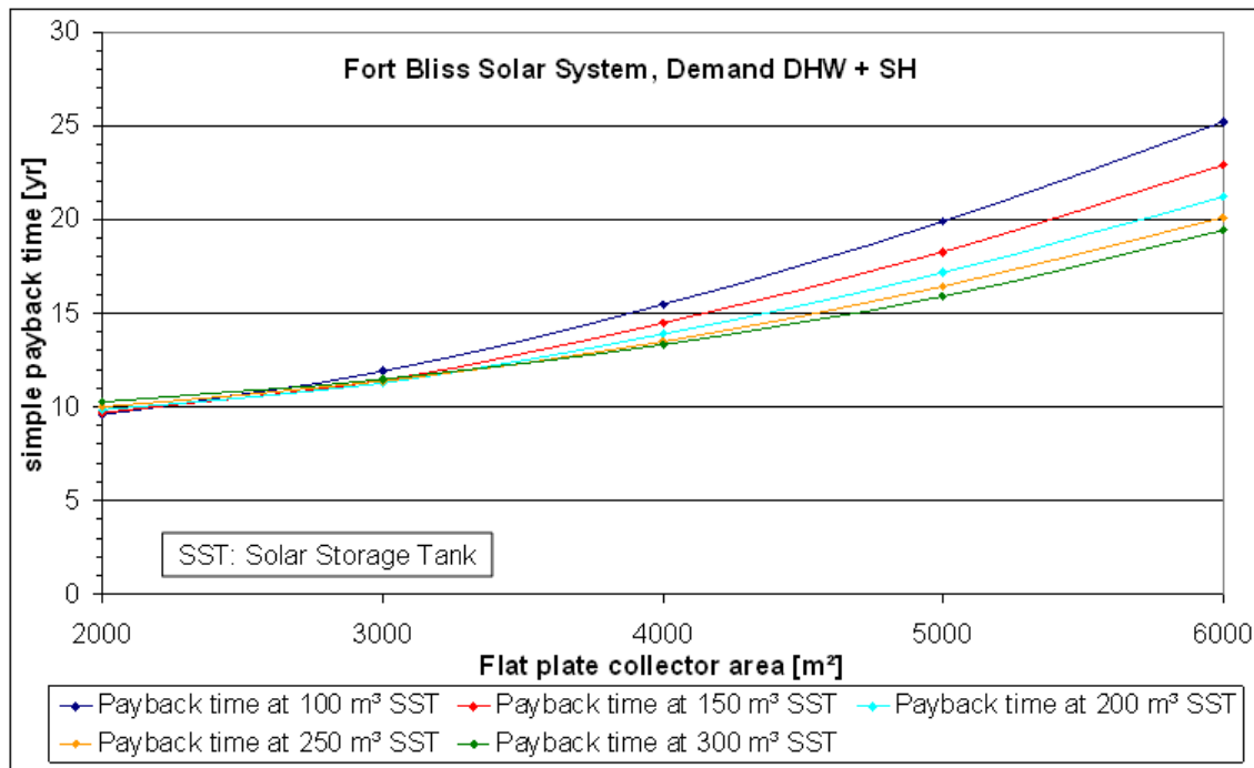
Figure B-28. Simple payback time depending on flat plate area, Fort Bliss, DHW and space heating.
