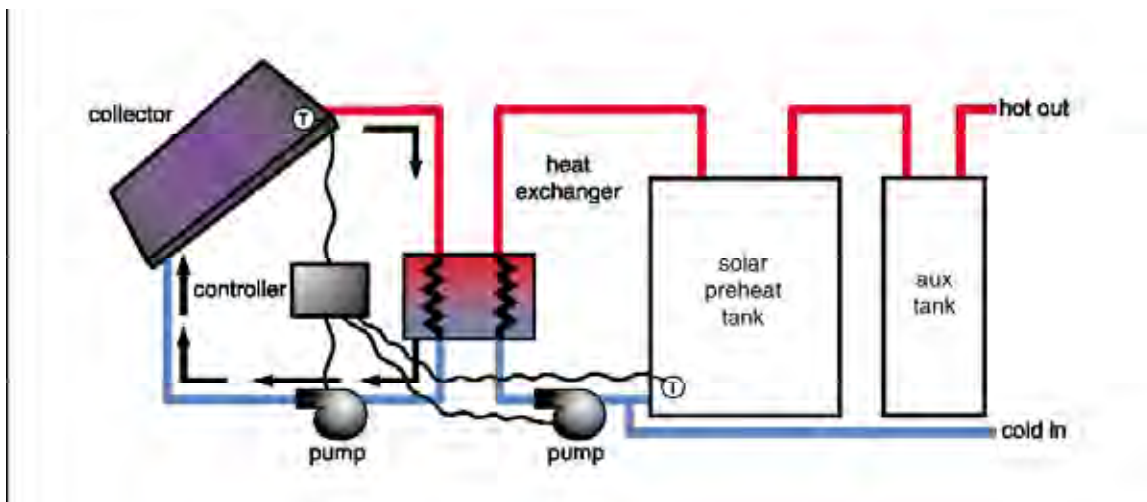
Figure 3.7. Schematic of an indirect active system that uses a heat exchanger to transfer heat from the collector to the water in the storage tank. These systems offer excellent freeze protection, tolerate hard water well, and have high maintenance requirements.
