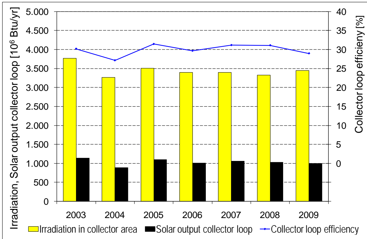
Figure A-57. Irradiation in collector area, solar energy output from collector loop, and collector loop efficiency.
