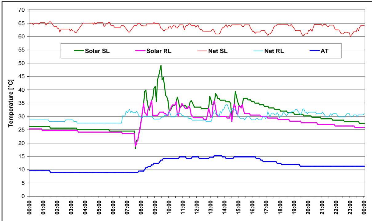
Figure A-8. Temperatures of the solar loop and the distribution grid in March 23 rd 2001, Gneis-Moos.
