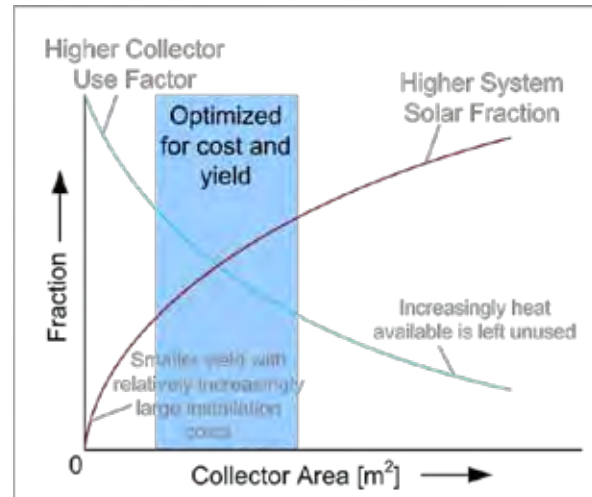
Figure 4.5. Sizing is a compromise between costs and yield.
