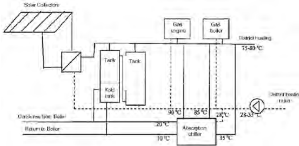
Figure A-23. Diagram of district heating system.
