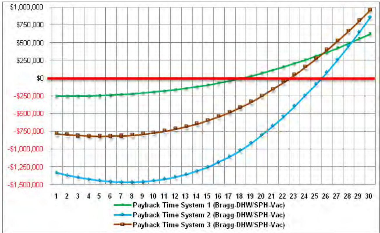
Figure B-36. Payback time - Fort Bragg – DHW / SPH – vacuum tube collectors.
