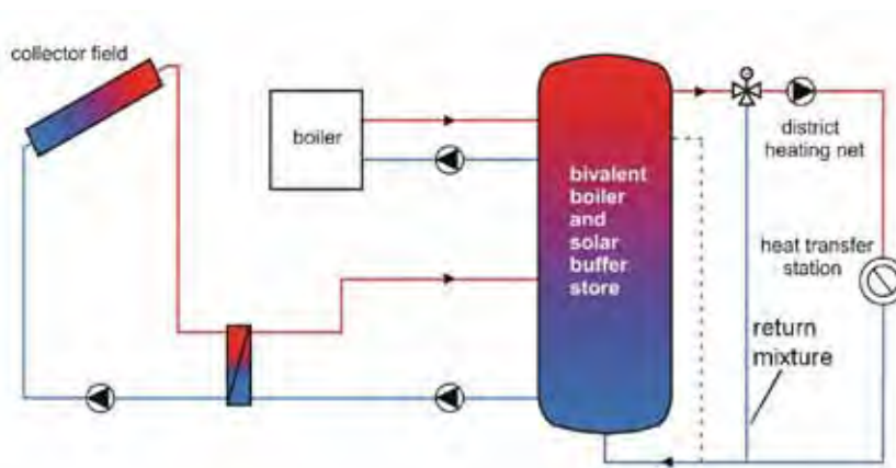
Figure A-43. Heating net with four-pipe boiler reheating inside buffer store.
