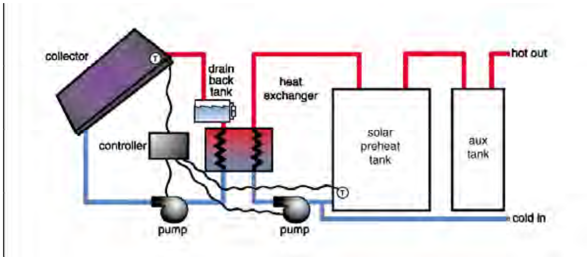
Figure 3.6. An active, drainback solar water heating system. These systems offer good freeze and overheat protection, tolerate hard water well, and have high maintenance requirements.
